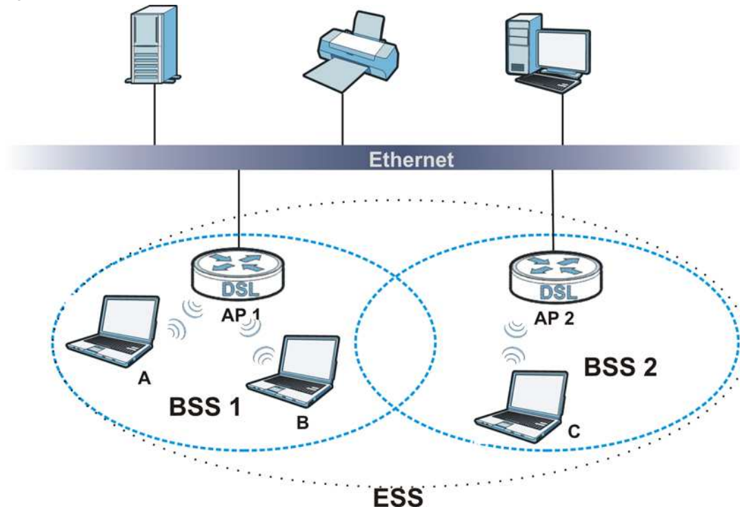
Figure 253 Infrastructure WLAN
