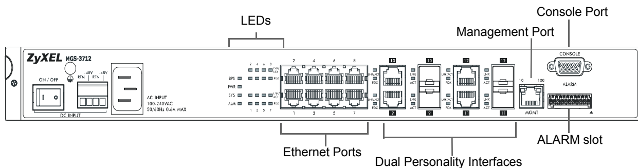
Figure 8 Front Panel: MGS-3712 AC/DC version
