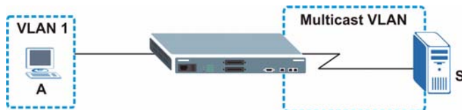
Figure 90 MVR Multicast Television Example
