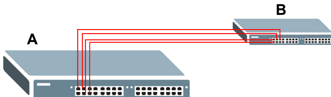
Figure 70 Trunking Example - Physical Connections
