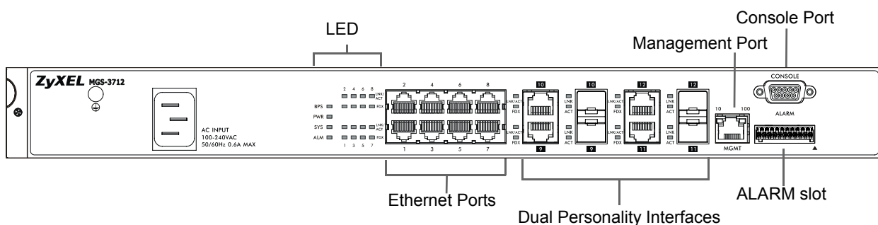
Figure 9 Front Panel: MGS-3712 AC version
