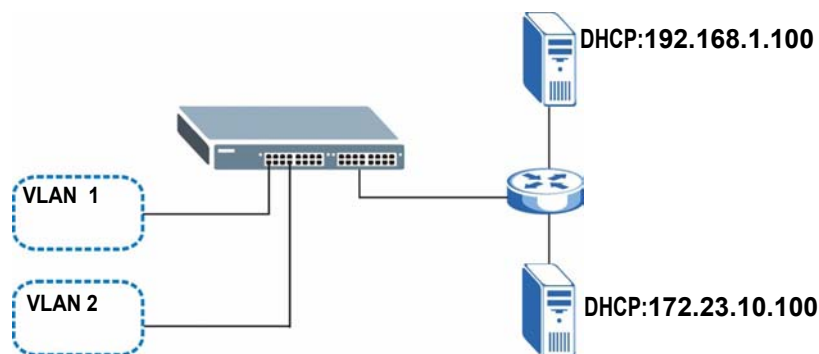
Figure 133 DHCP Relay for Two VLANs
