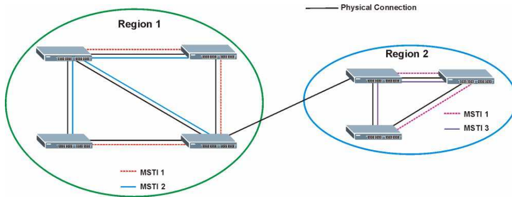
Figure 54 MSTIs in Different Regions
