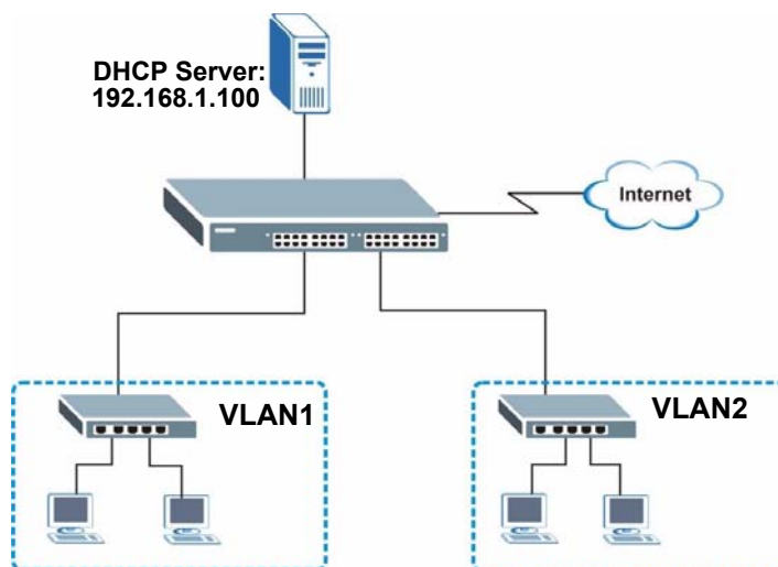
Figure 130 Global DHCP Relay Network Example
