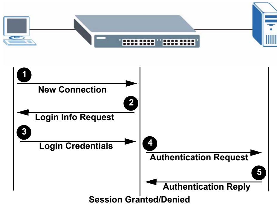
Figure 72 IEEE 802.1x Authentication Process
