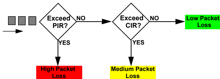
Figure 123 trTCM - Color-blind Mode
