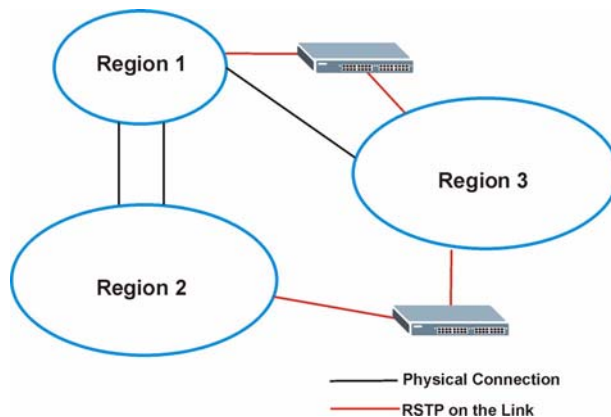
Figure 55 MSTP and Legacy RSTP Network Example
