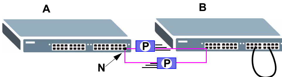
Figure 118 Loop Guard - Probe Packet
