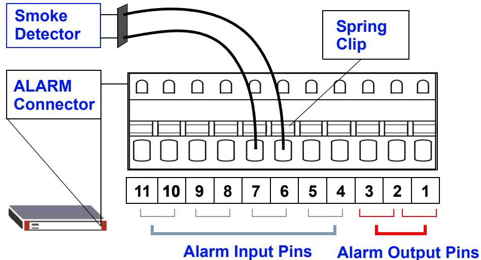
Figure 20 Connecting a Sensor to the ALARM Slot
