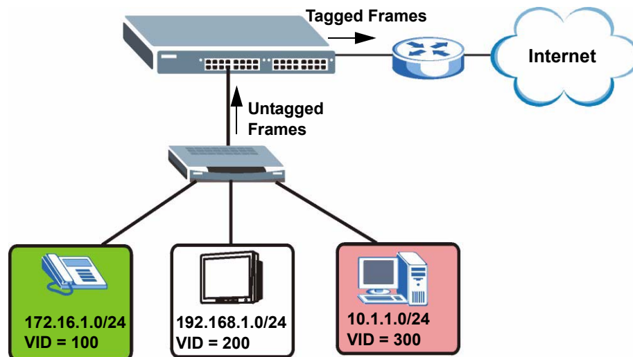
Figure 45 Subnet Based VLAN Application Example
