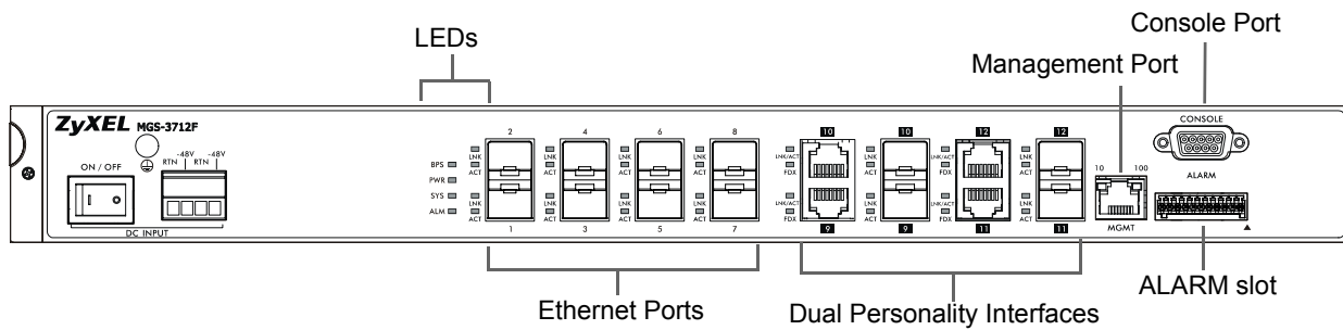
Figure 13 Front Panel: MGS-3712F DC version
