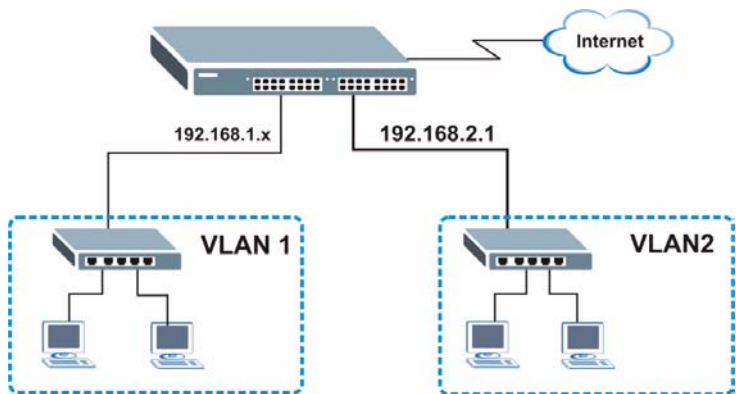
Figure 31 Initial Setup Example: Management IP Address
