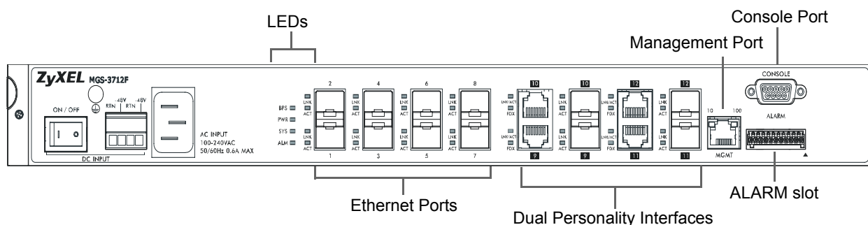
Figure 11 Front Panel: MGS-3712F AC/DC version
