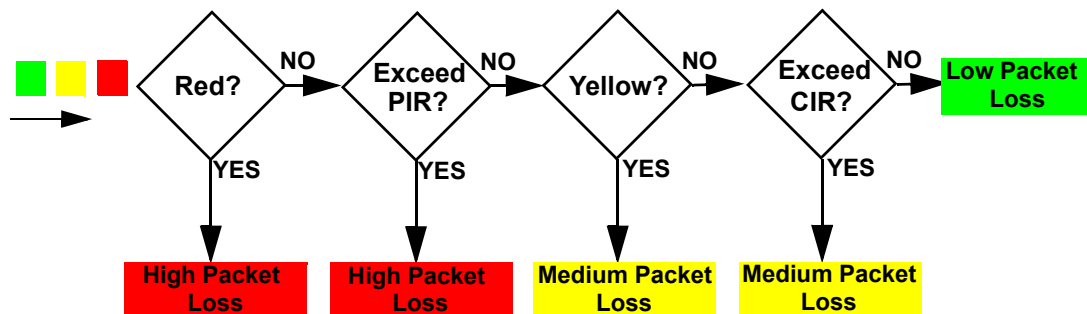
Figure 124 trTCM - Color-aware Mode
