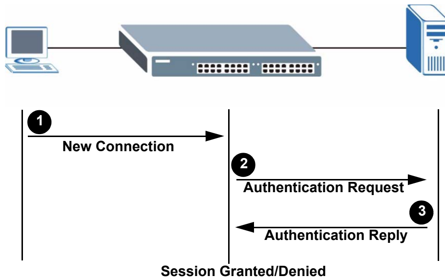
Figure 73 MAC Authentication Process
