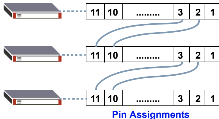
Figure 21 Daisy-chaining an External Alarm Sensor to Other MGS-3712s
