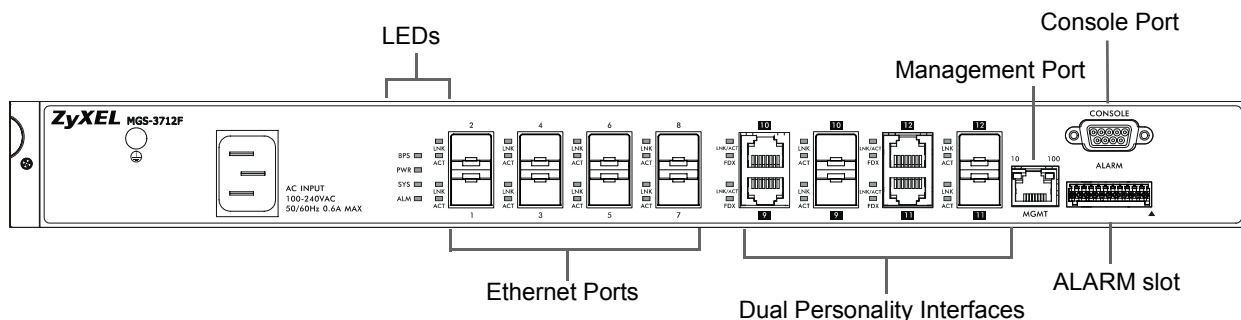
Figure 12 Front Panel: MGS-3712F AC version
