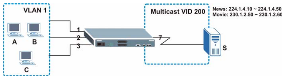
Figure 93 MVR Configuration Example
