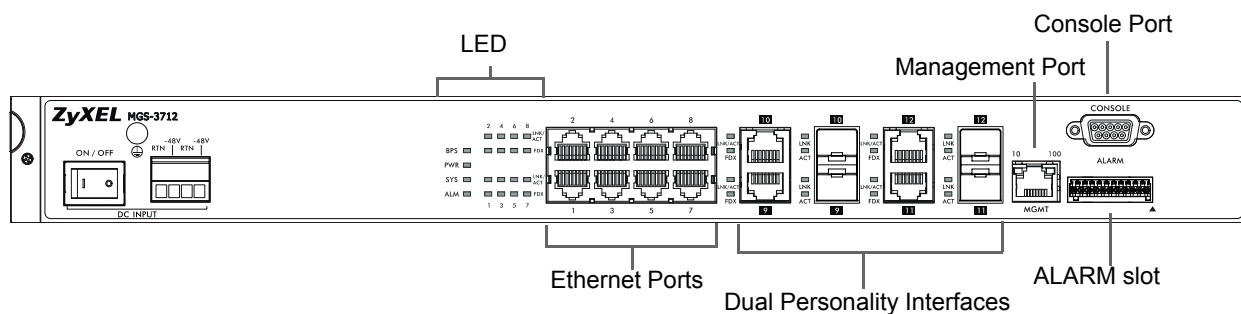
Figure 10 Front Panel: MGS-3712 DC version
