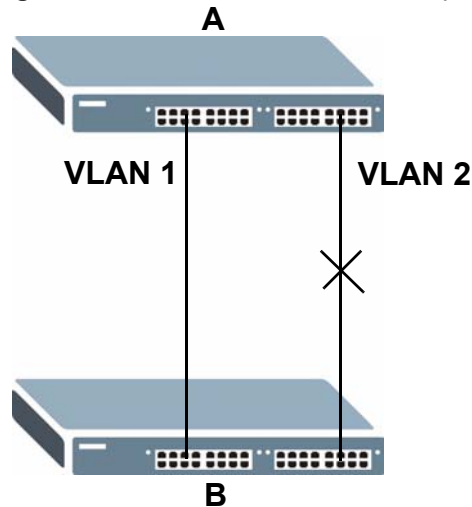
Figure 52 STP/RSTP Network Example
