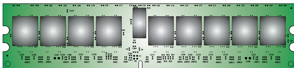
SOLDER SIDE—MIRRORED
