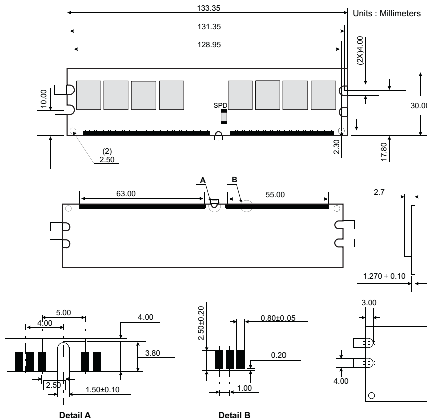
Figure 1: KVR667D2N5/512 240-Pin DIMM
