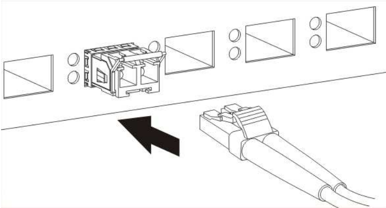
Figure 12 Connecting the Fiber Optic Cables
