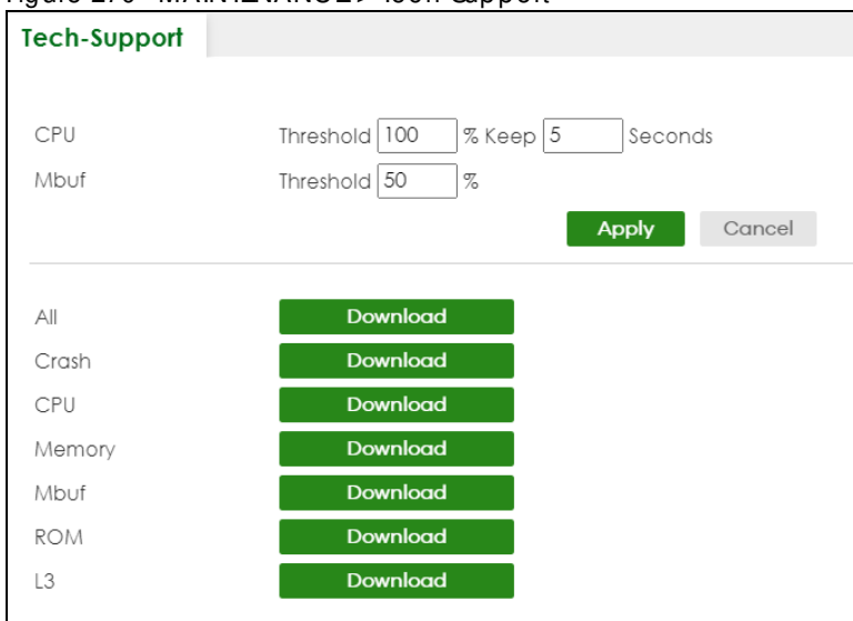
Figure 270 MAINTENANCE &gt; Tech-Support
