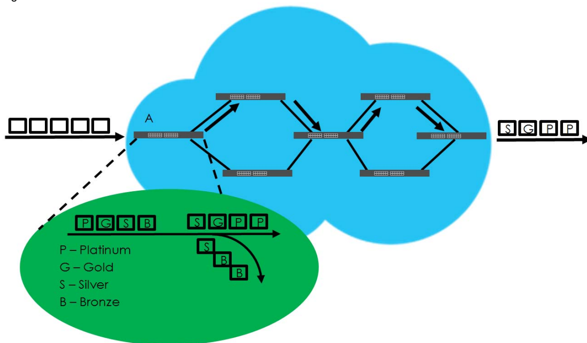
Figure 164 DiffServ Network
