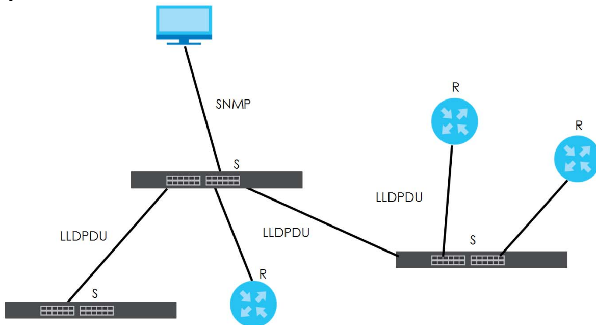
Figure 128 LLDP Overview
