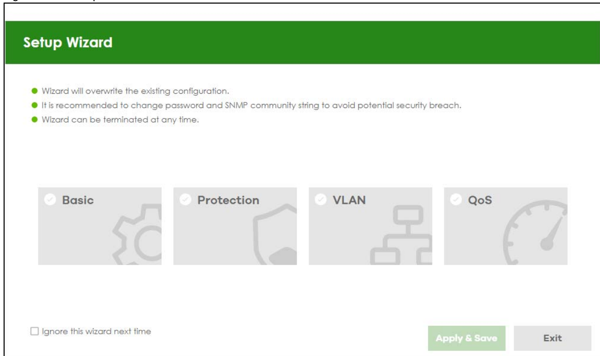
Figure 35 Setup Wizard
