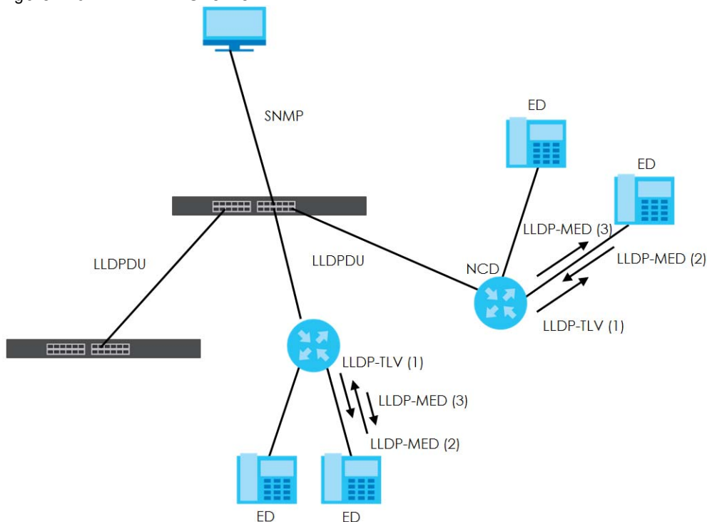
Figure 129 LLDP-MED Overview
