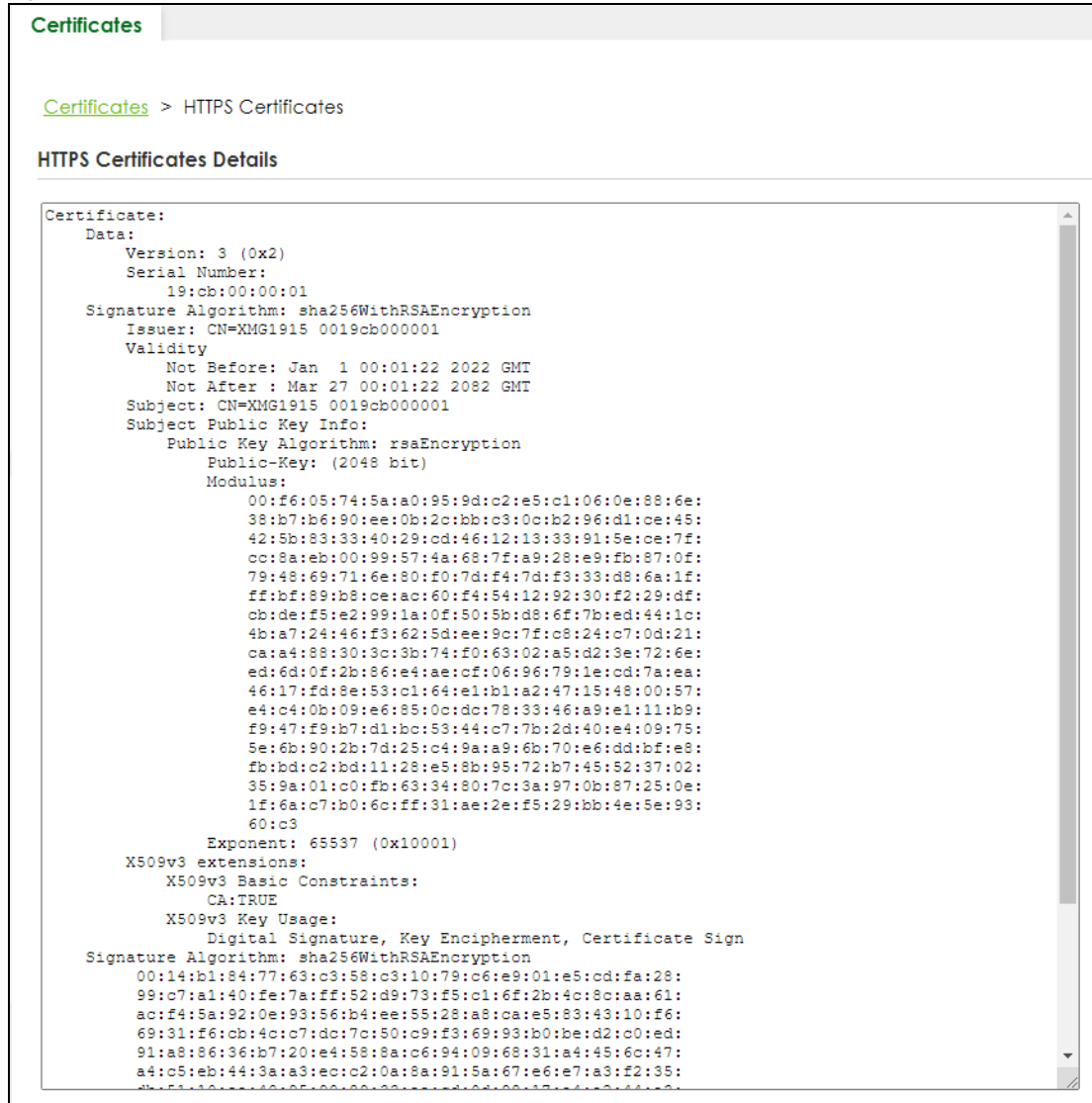
Figure 252 MAINTENANCE &gt; Certificates &gt; HTTPS
