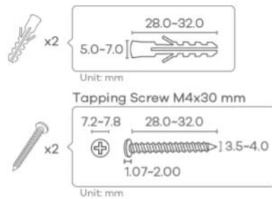
Figure 6 Screw Specifications
