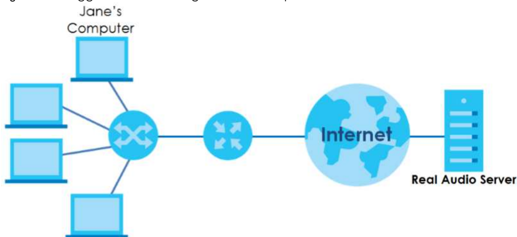
Figure 49 Trigger Port Forwarding Process: Example
