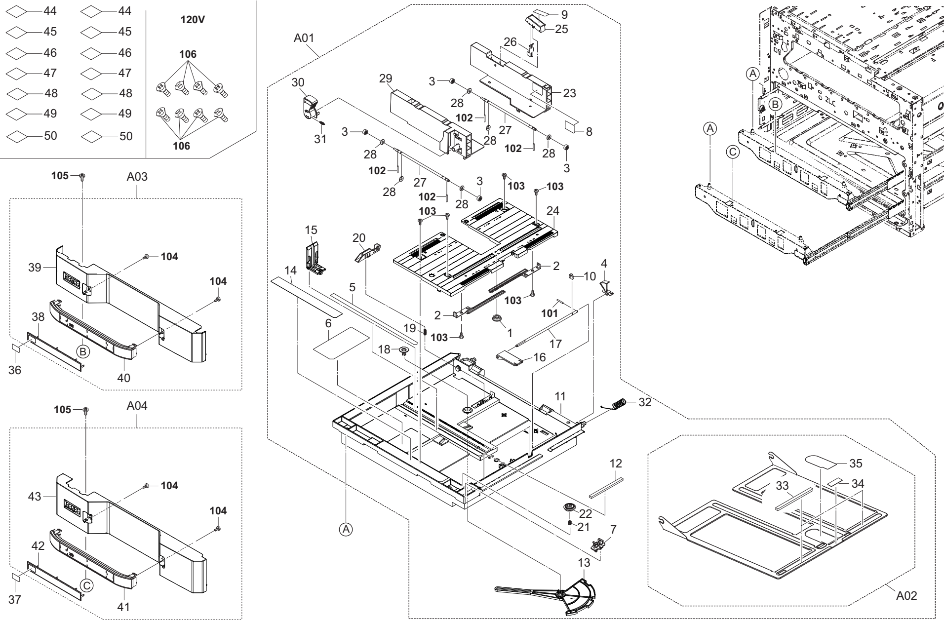
FIG. 6 Paper Cassettes
