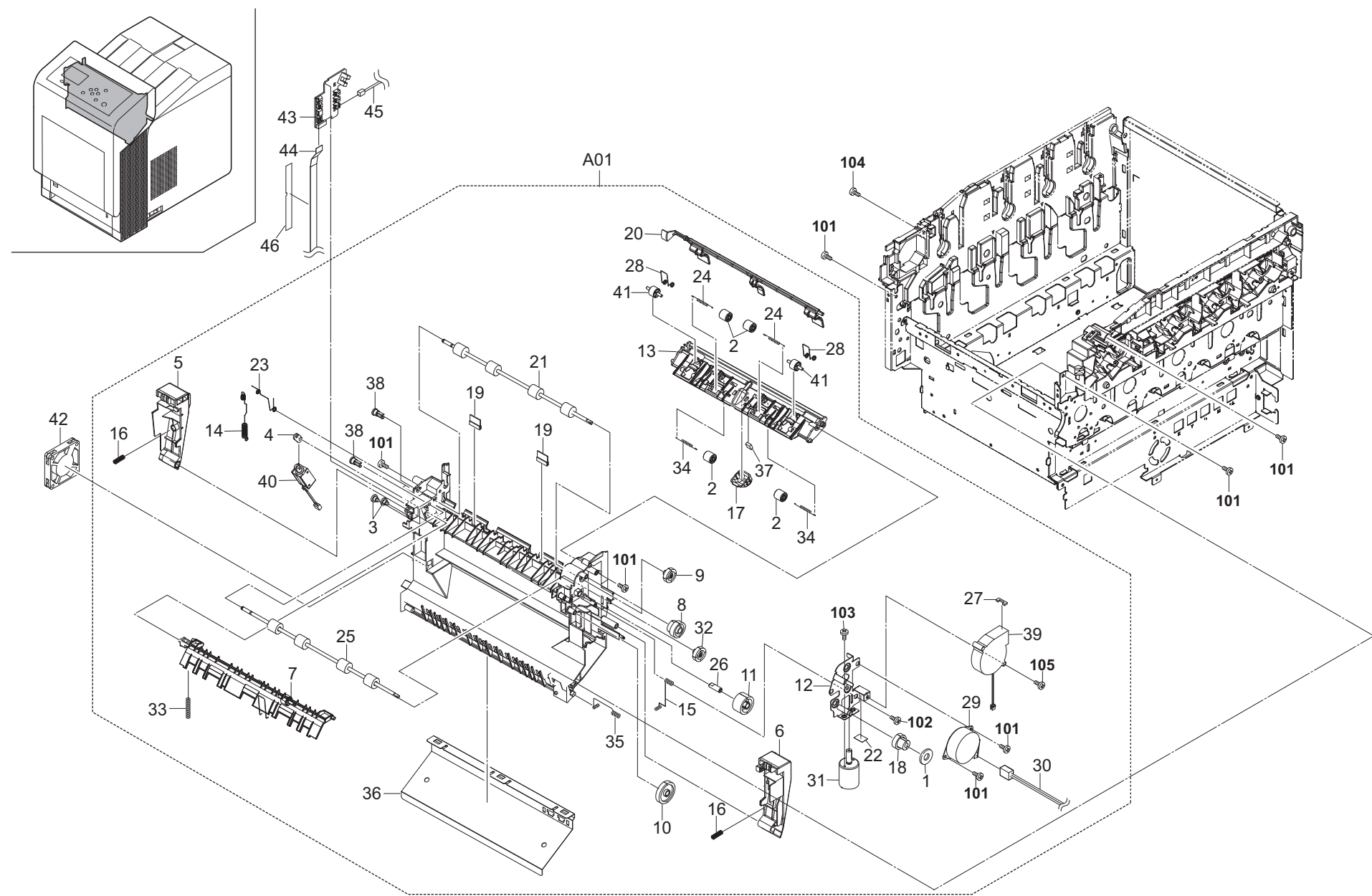
FIG. 13 Exit Section
