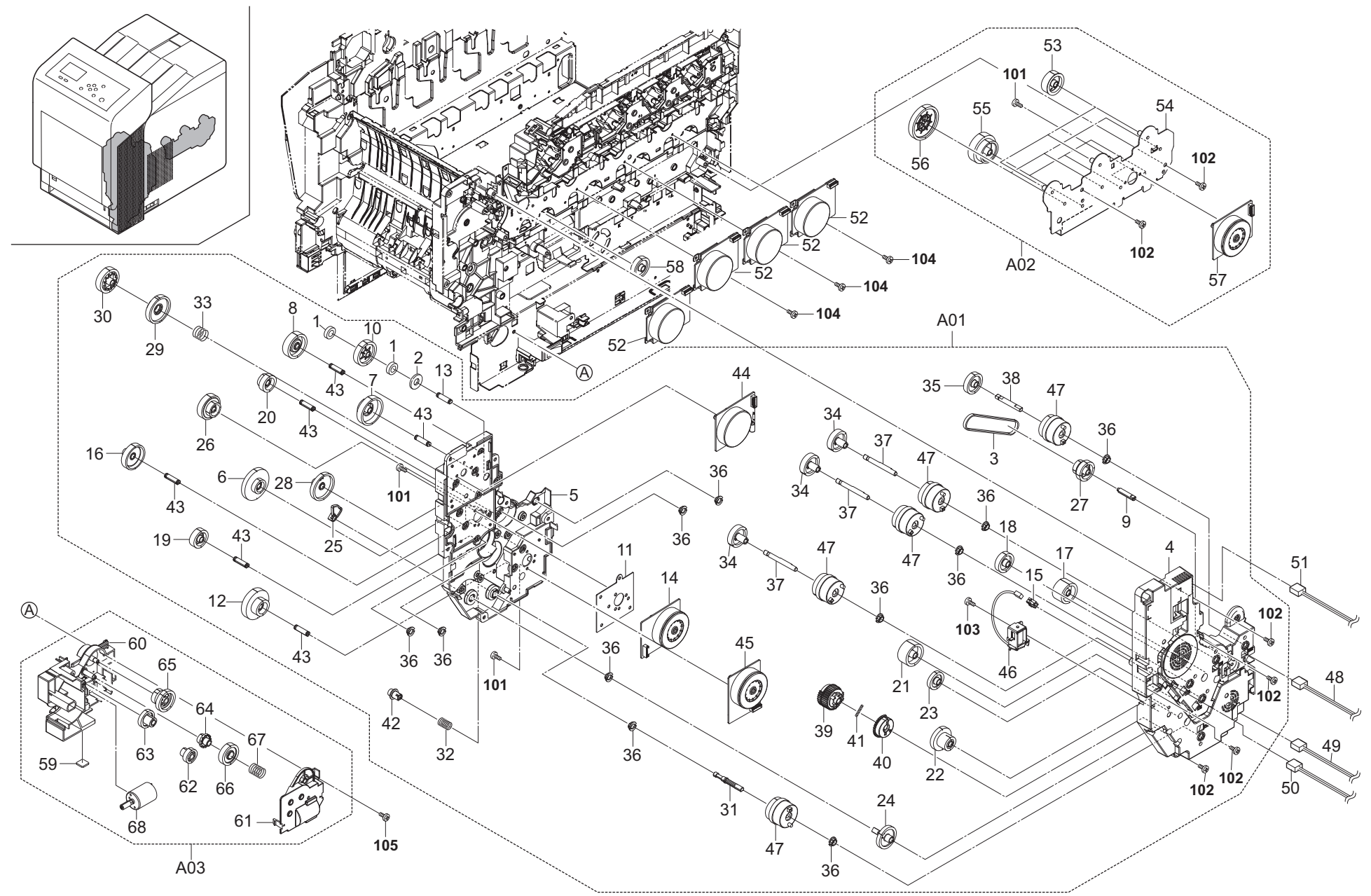
FIG. 12 Drive Section
