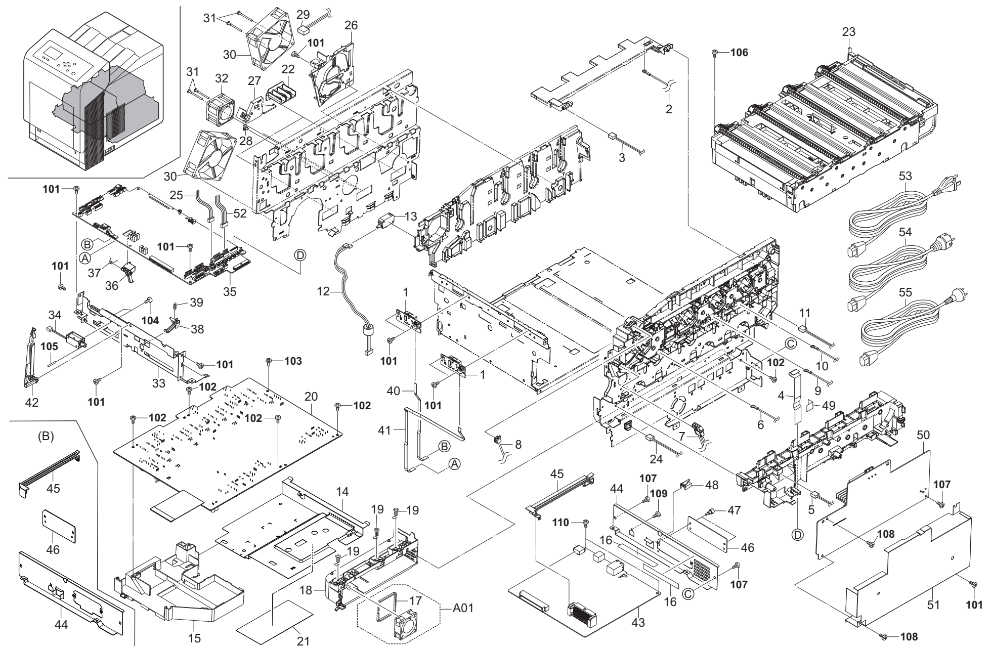
FIG. 14 Electrical Components
