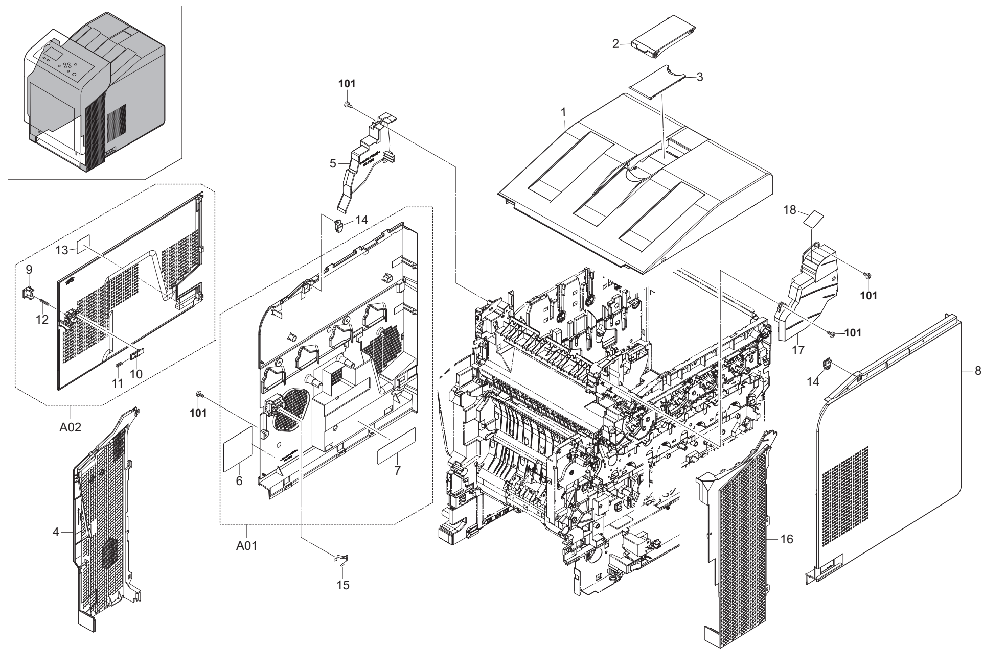
FIG. 1 Covers 1
