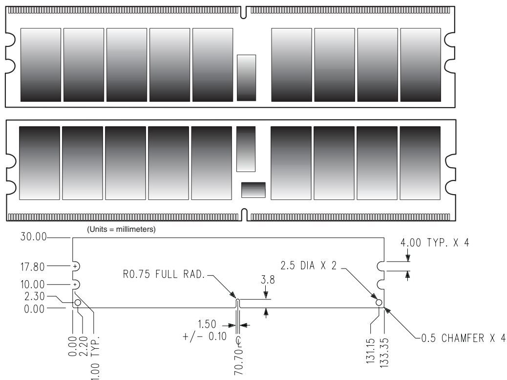
Figure 1: KVR400D2S4R3/1GI 240-Pin DIMM
