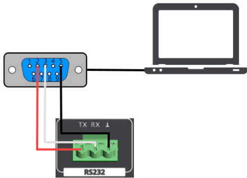
Figure 18. RS232 Wiring
