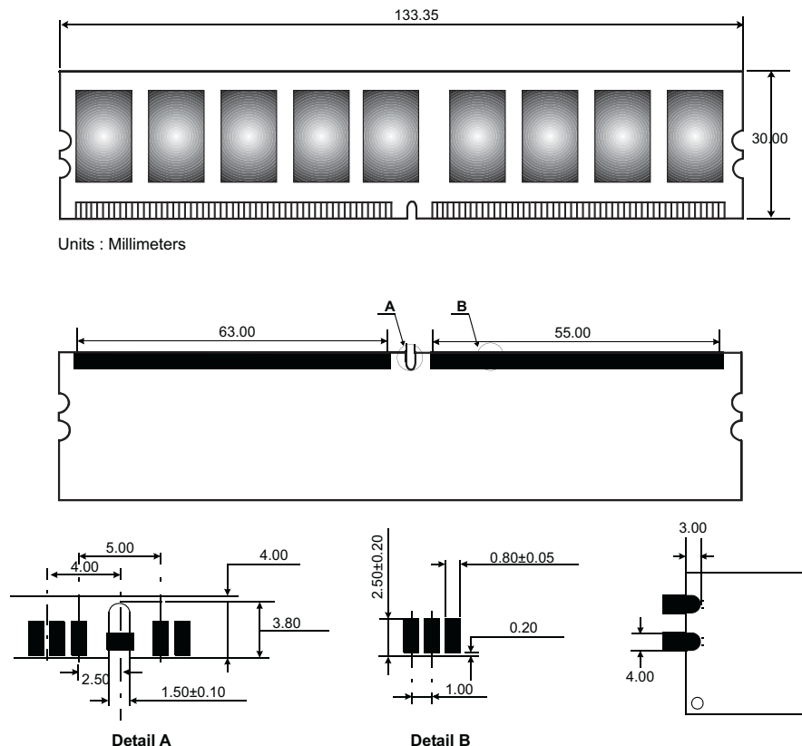
Figure 1: KVR667D2E5/512 240-Pin DIMM
