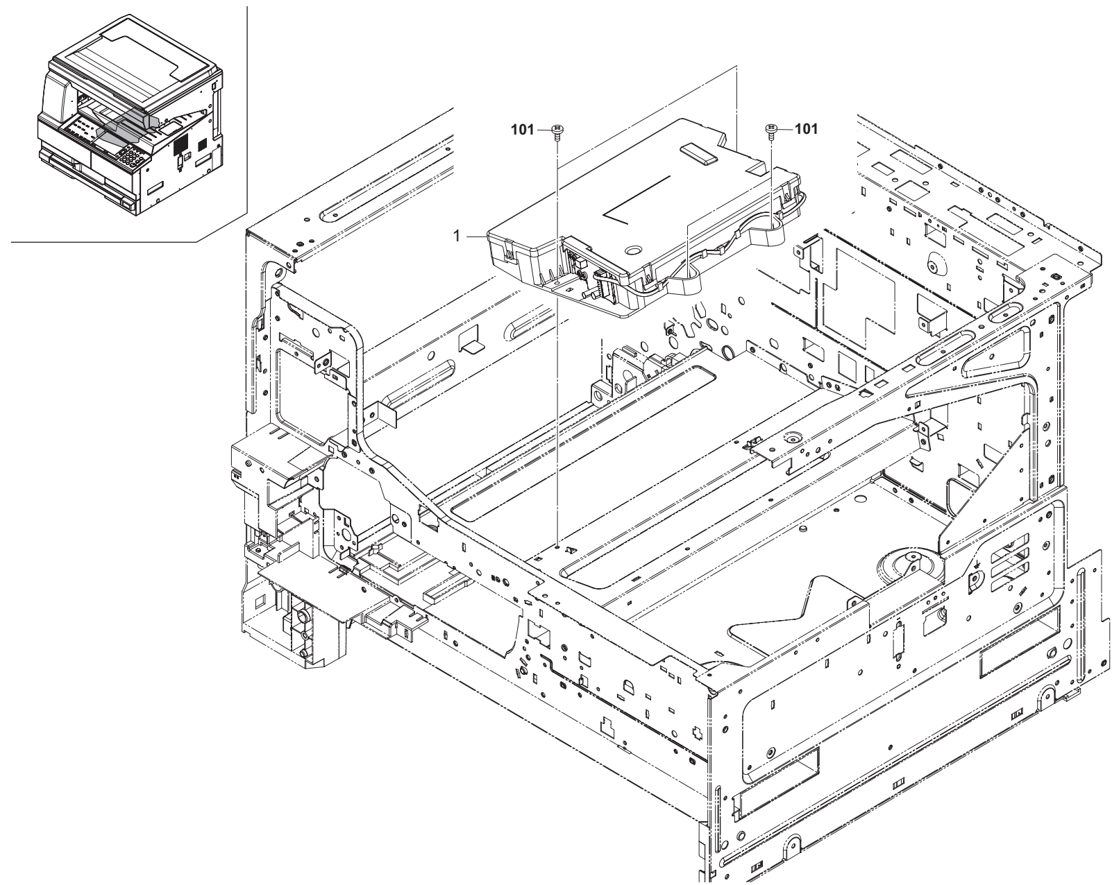
FIG. 9 Laser Scanner Section
