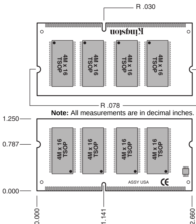
Figure 1: KVR133X64SC3/64 144-Pin SDRAM Module
