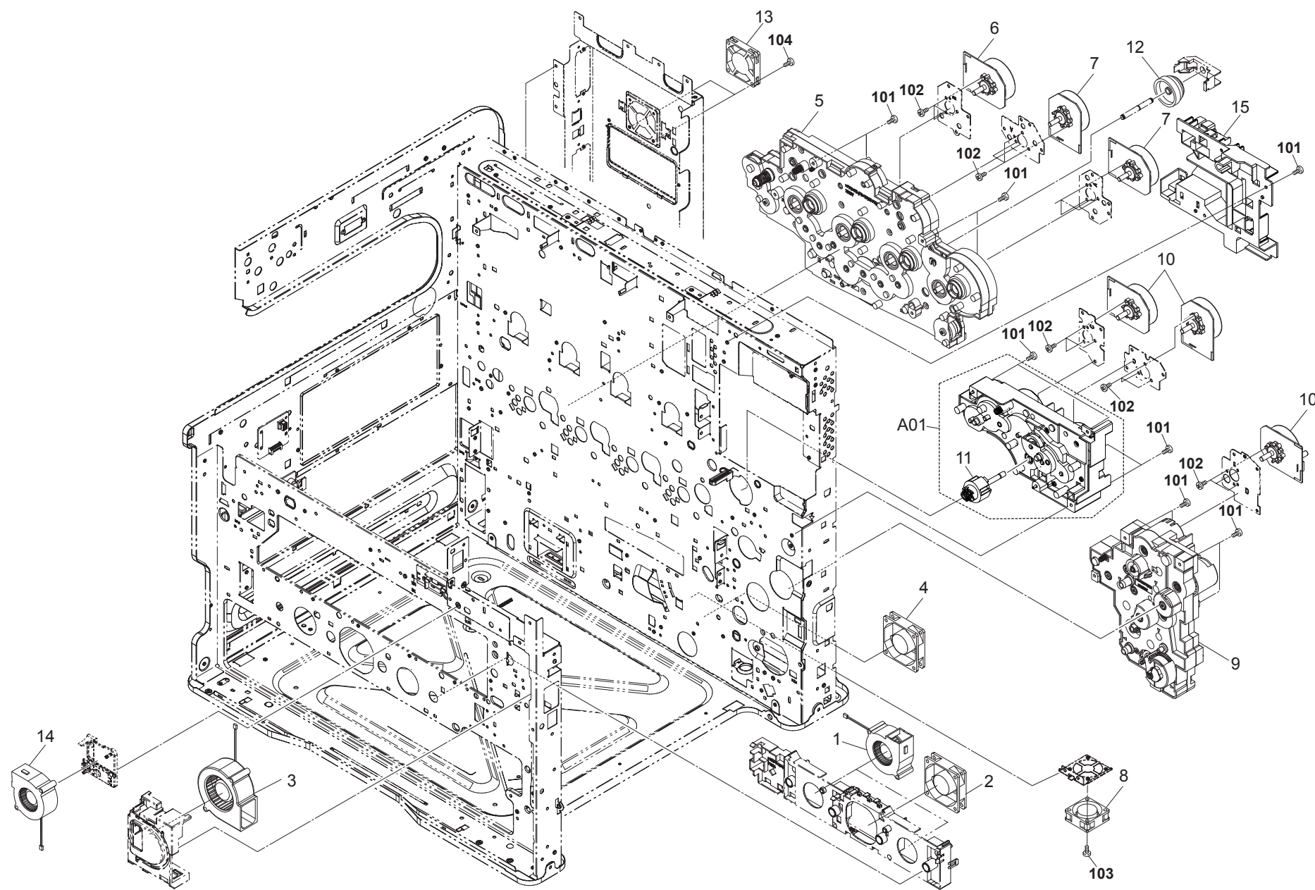
FIG. 14 Drive Section
