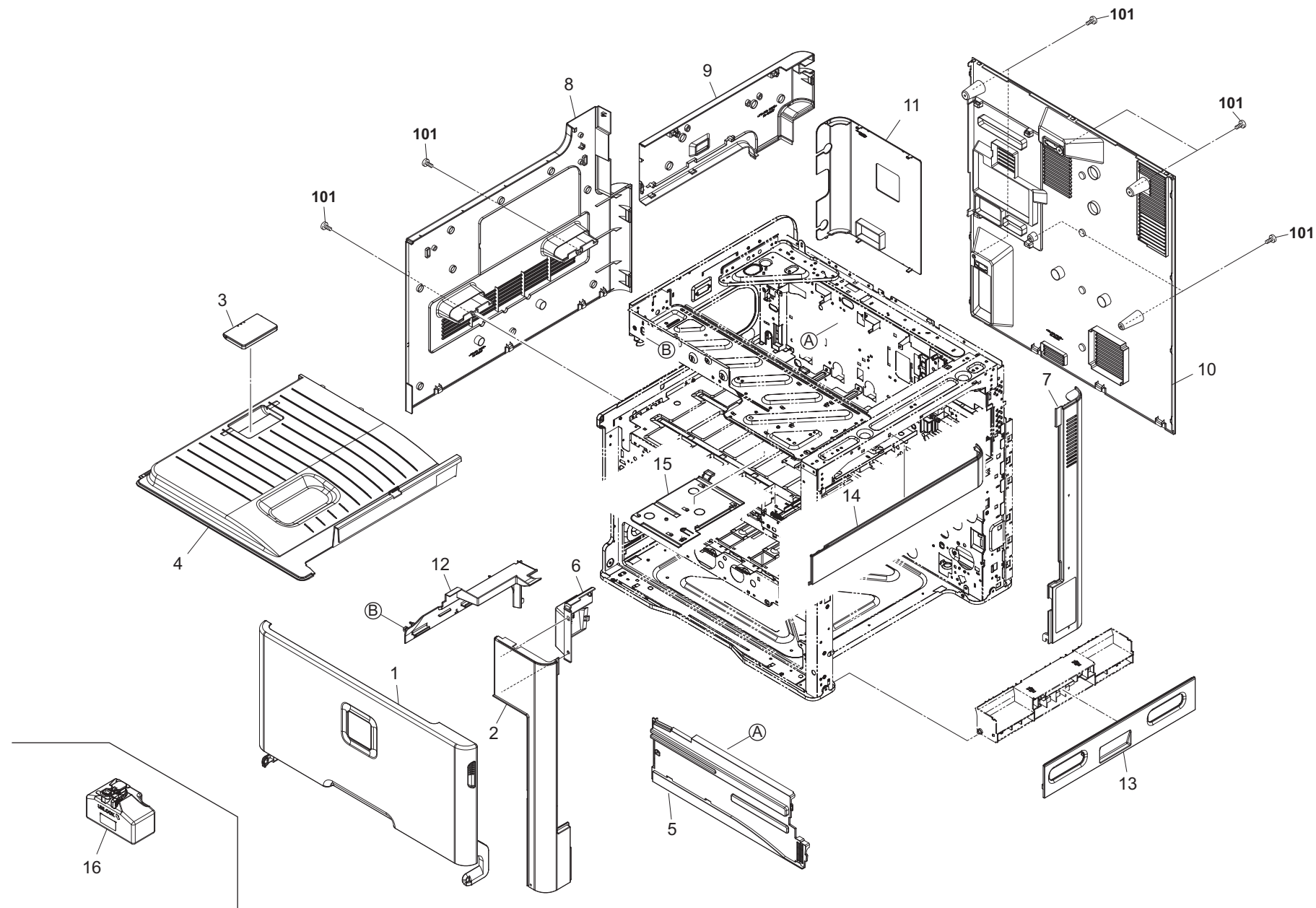
FIG. 1 Covers
