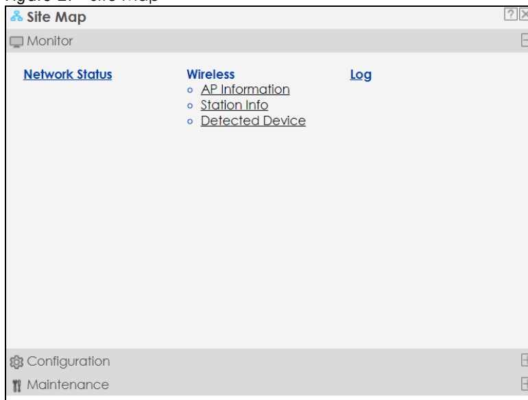
Figure 27 Site Map
