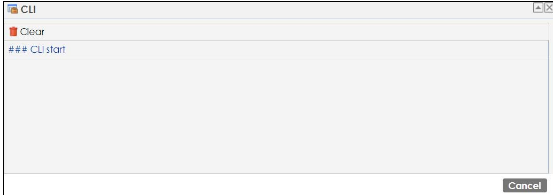
Figure 28 CLI Messages
