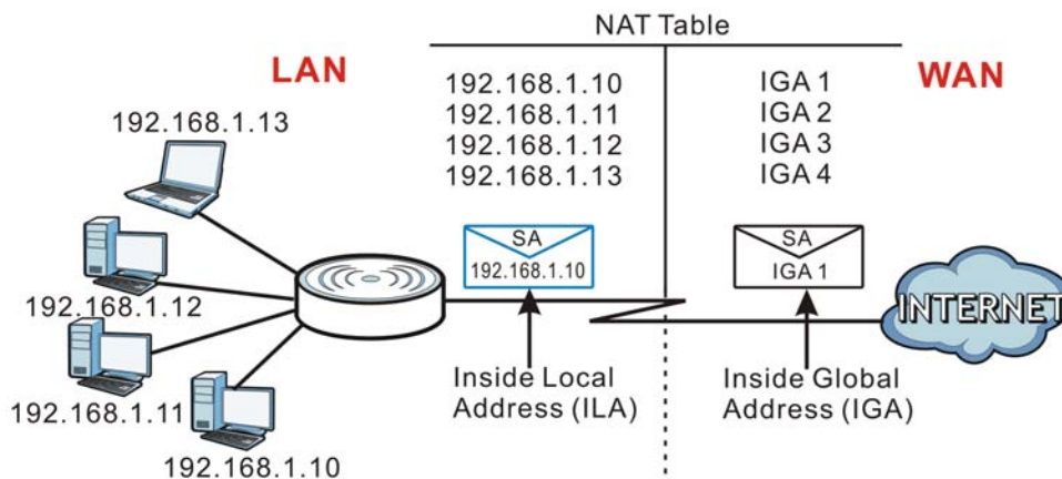
Figure 75 How NAT Works
