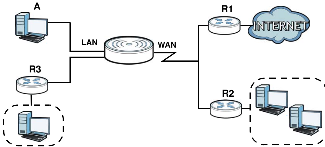
Figure 82 Example of Static Routing Topology
