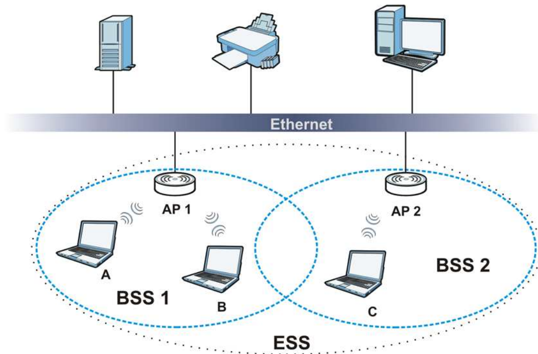
Figure 145 Infrastructure WLAN
