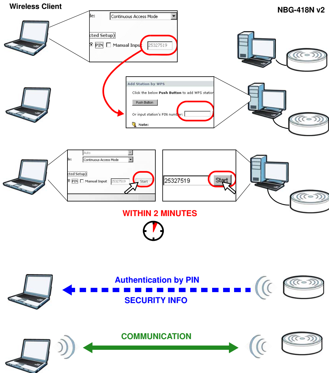
Figure 33 Example WPS Process: PIN Method
