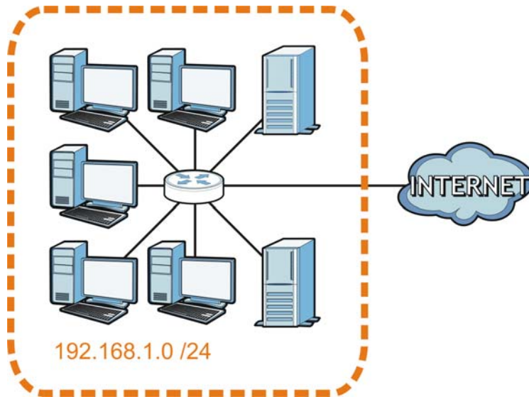
Figure 119 Subnetting Example: Before Subnetting
