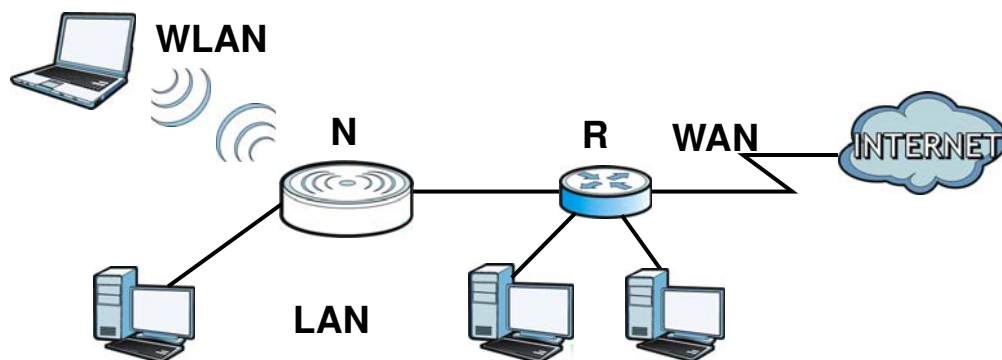
Figure 18 AP Mode
