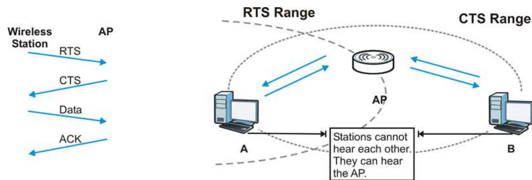
Figure 146 RTS/CTS
