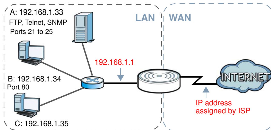
Figure 74 NAT Example
