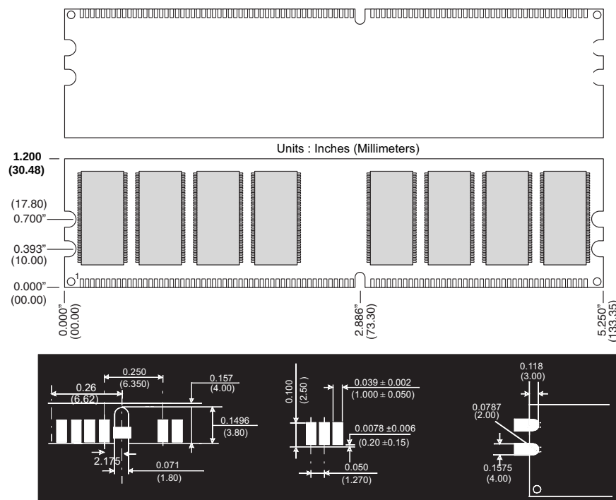
Figure 1: KVR333X64C25/256 184-Pin DDR SDRAM Module
