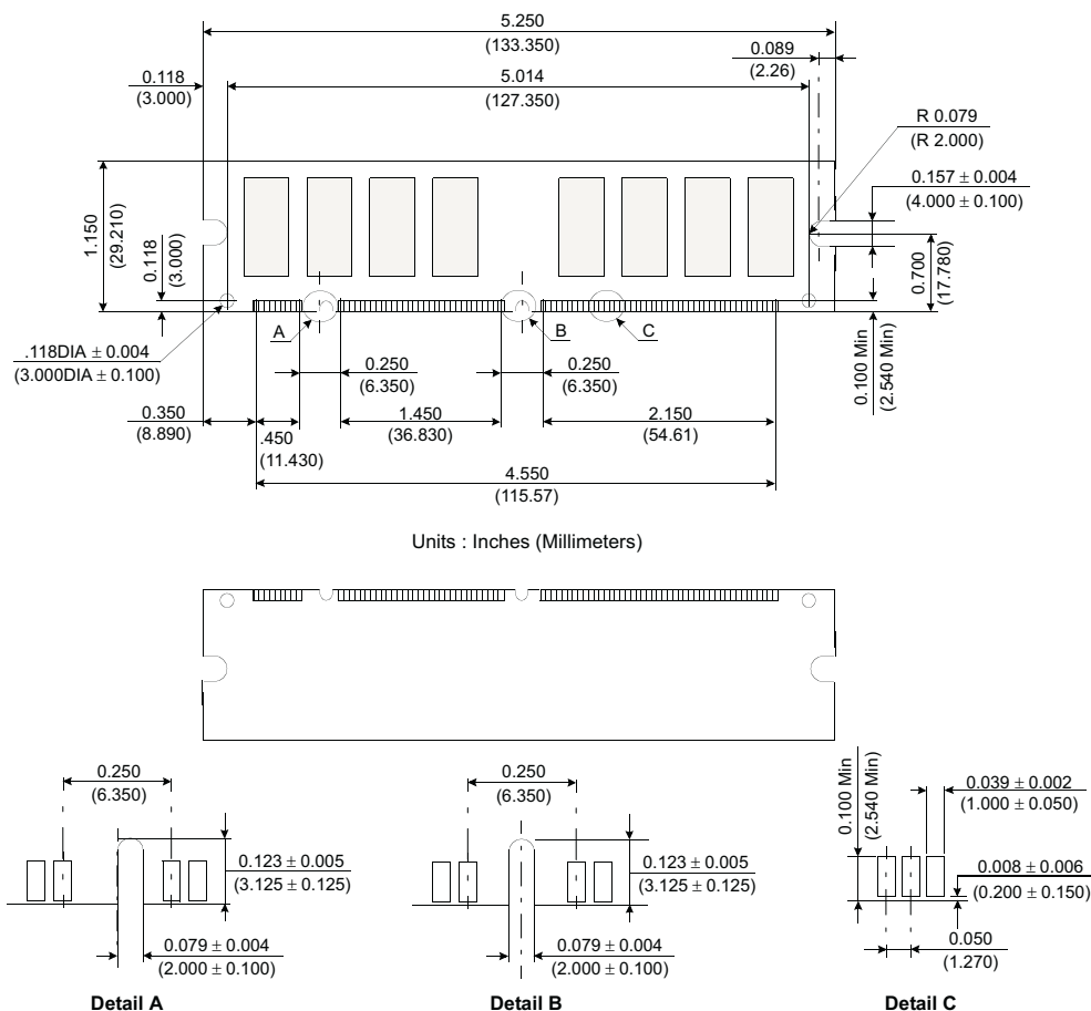
Figure 1: KVR133X64C3L/256 168-Pin SDRAM Module
