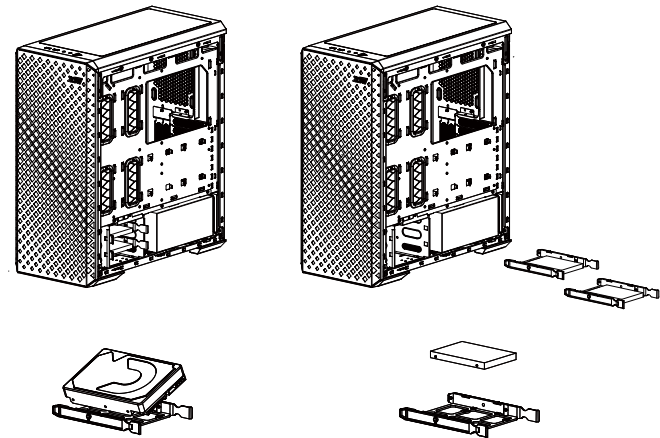
3.5" HDD Installation
