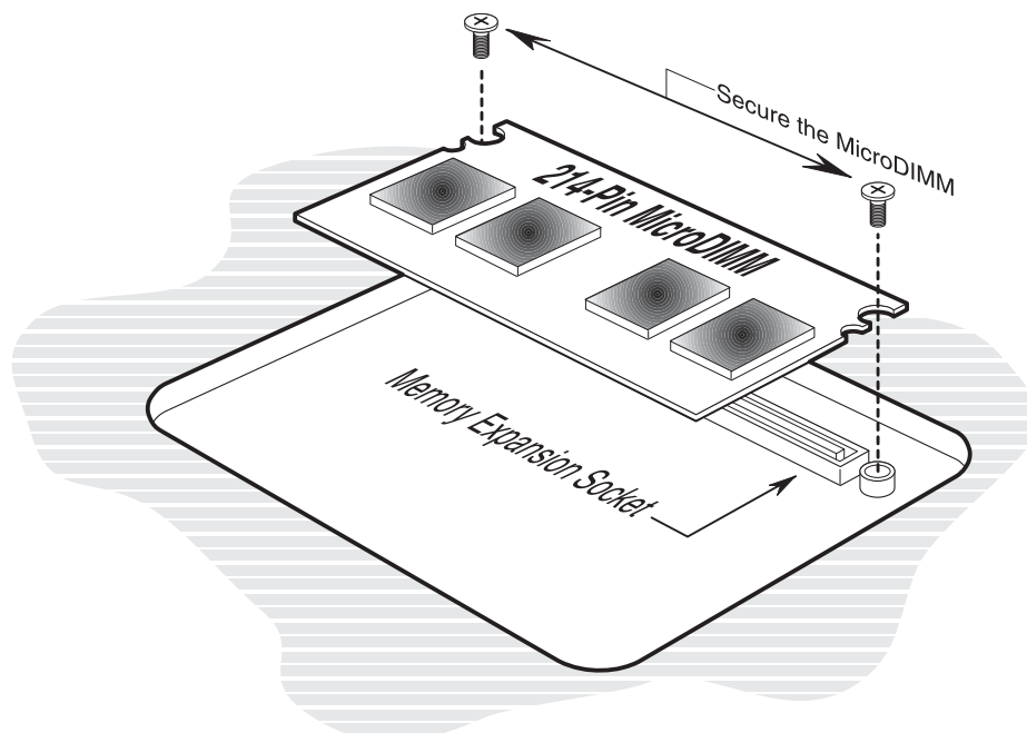
KVR533D2U4/512 214-Pin MicroDIMM
