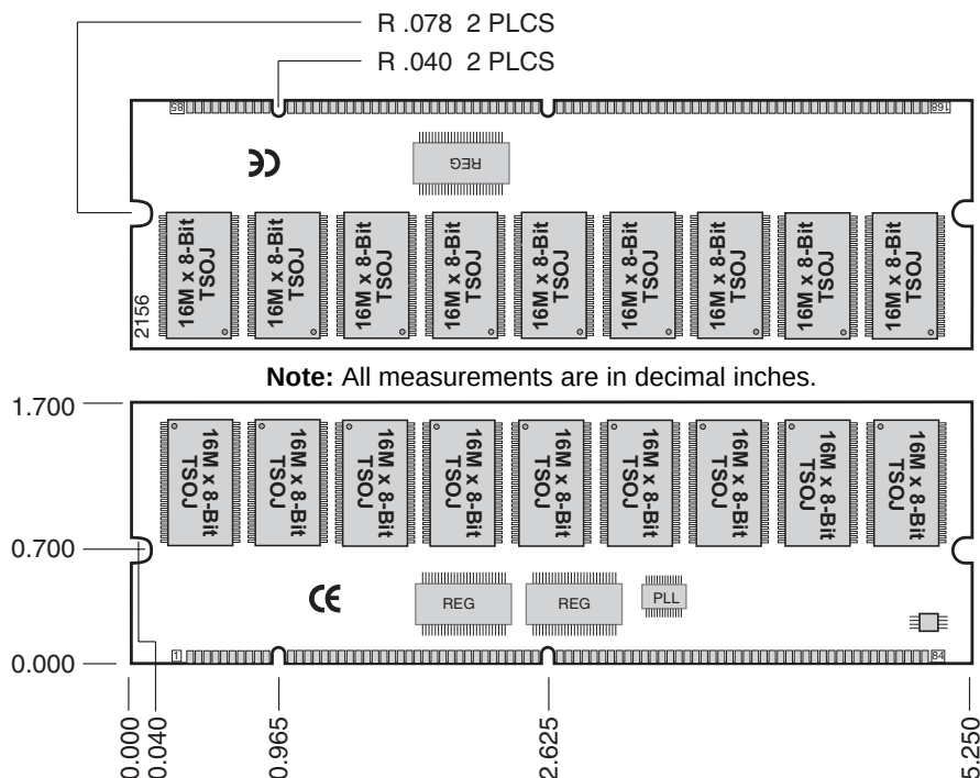
Figure 1: KVR100X72RC2/256 168-Pin SDRAM Module
