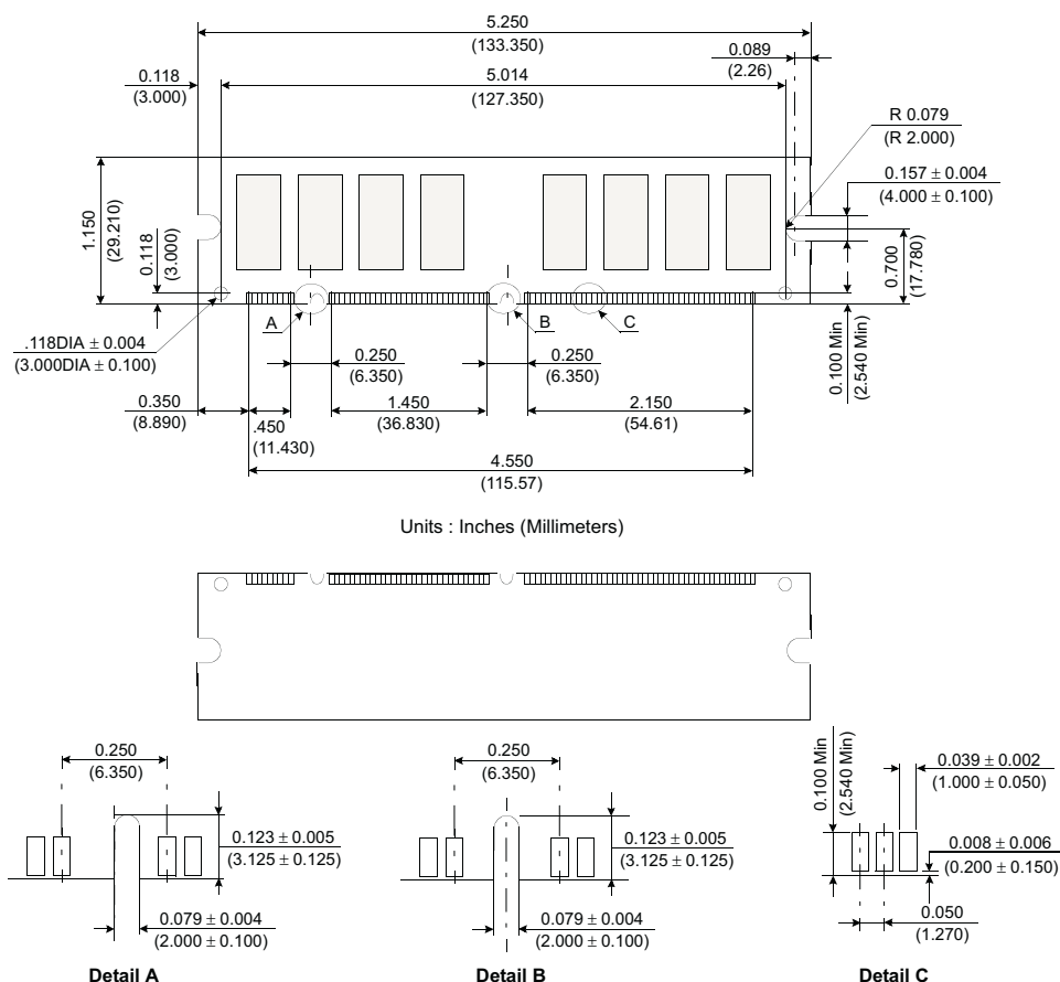
Figure 1: KVR133X64C3/256 168-Pin SDRAM Module
