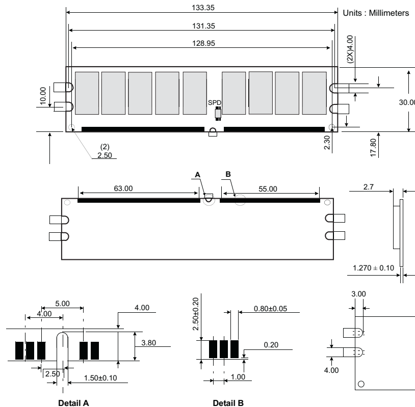
Figure 1: KVR400D2E3/512 240-Pin DIMM
