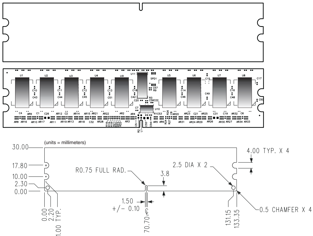
Figure 1: KVR400D2R3K2/1G 240-Pin DIMM
