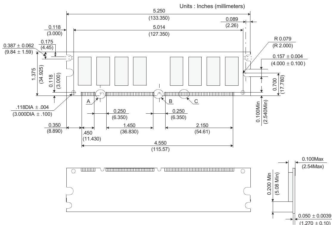
Figure 1: KVR100X64C3/64 168-Pin SDRAM Module
