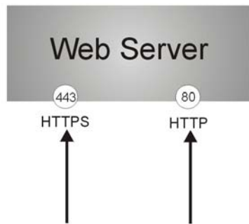
Figure 86 HTTP/HTTPS Implementation
