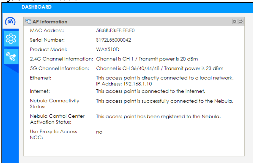
Figure 115 Dashboard
