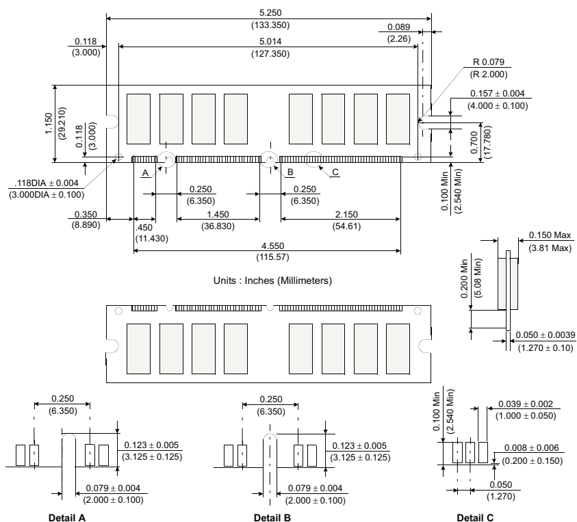
Figure 1: KVR133X64C3/256Q 168-Pin SDRAM Module
