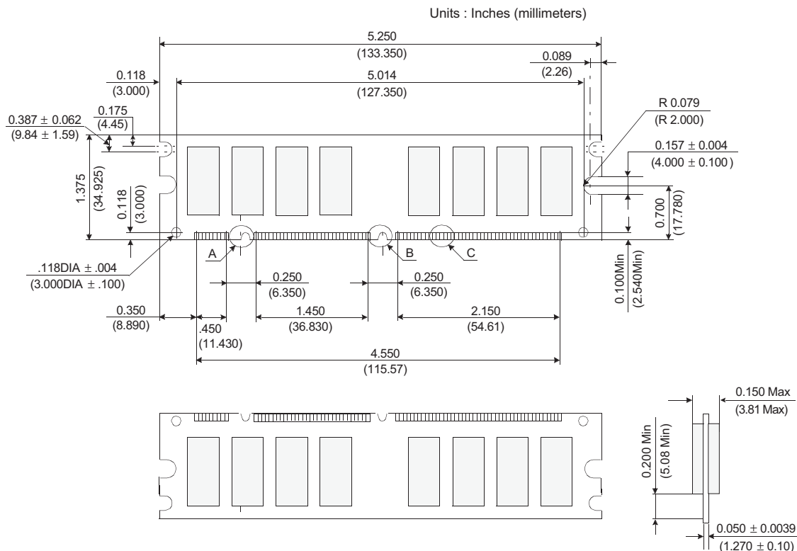
Figure 1: KVR100X64C3/128 168-Pin SDRAM Module
