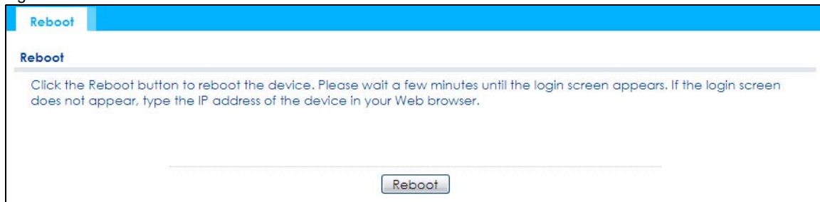
Figure 112 Maintenance > Reboot
