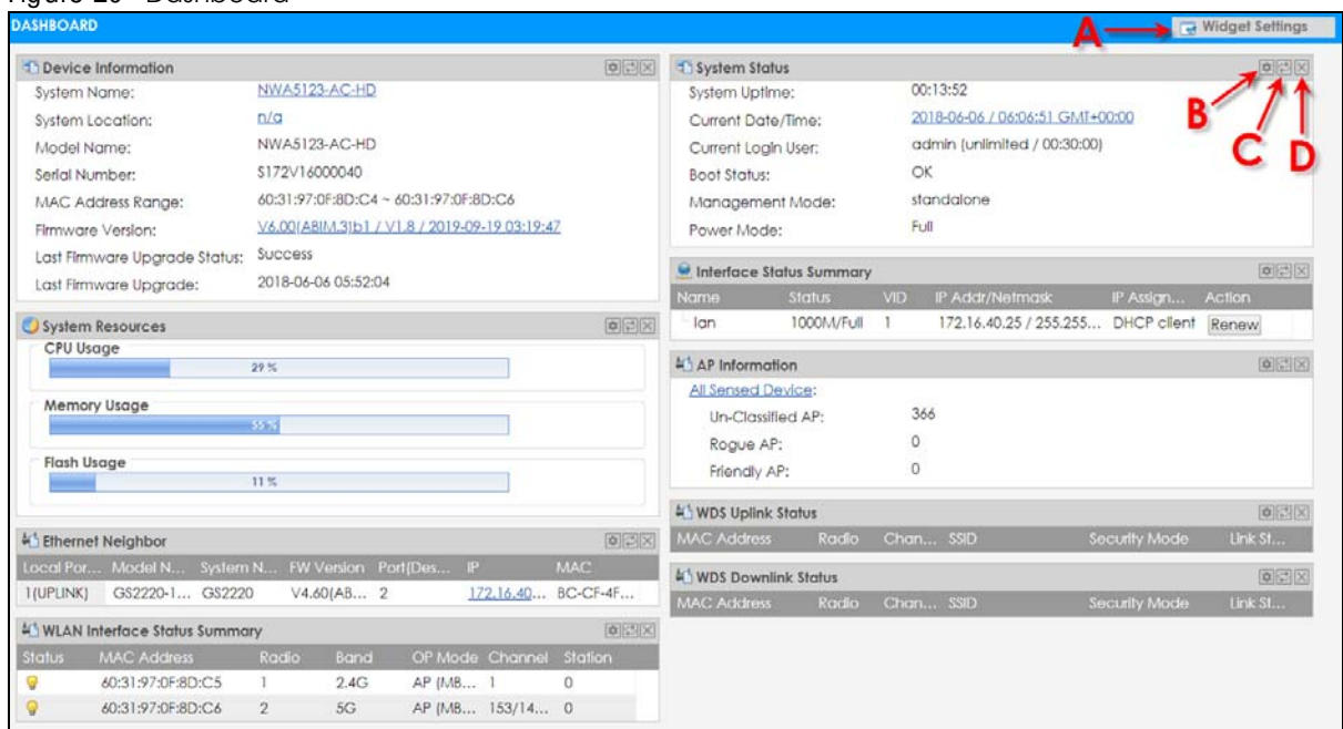
Figure 20 Dashboard
