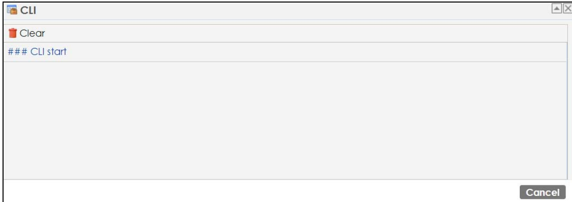
Figure 17 CLI Messages
