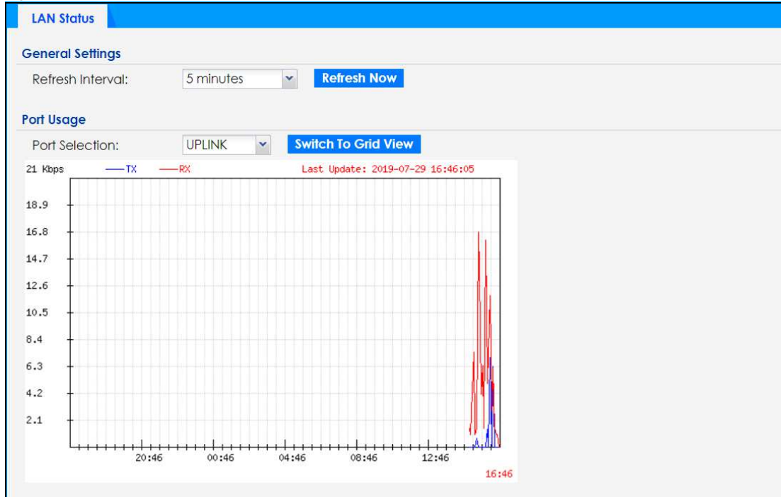
Figure 29 Monitor &gt; Network Status &gt; Switch to Graphic View
