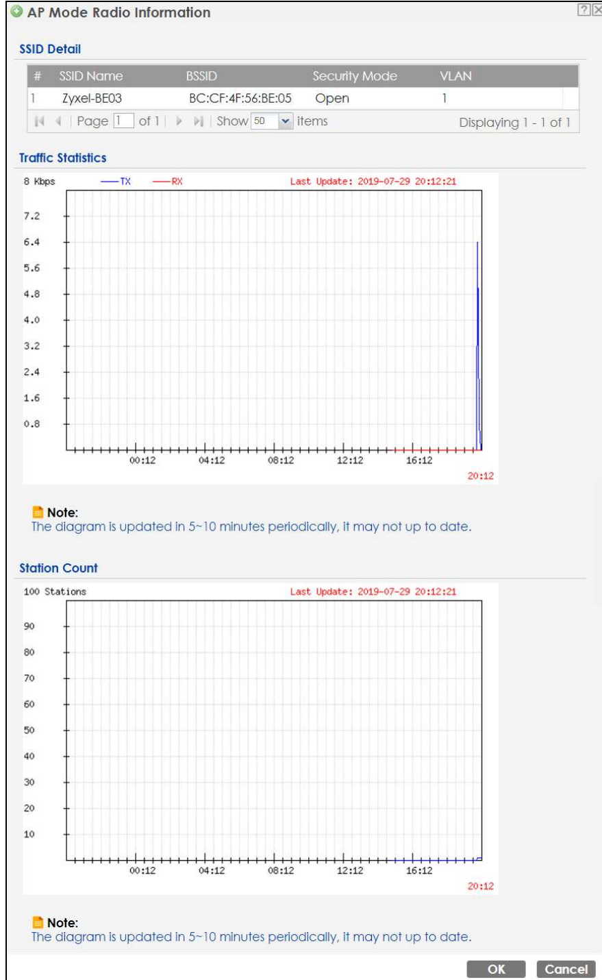
Figure 32 Monitor &gt; Wireless &gt; AP Information &gt; Radio List &gt; More Information
