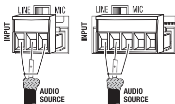
Figure 2.4.1 Input Wiring
