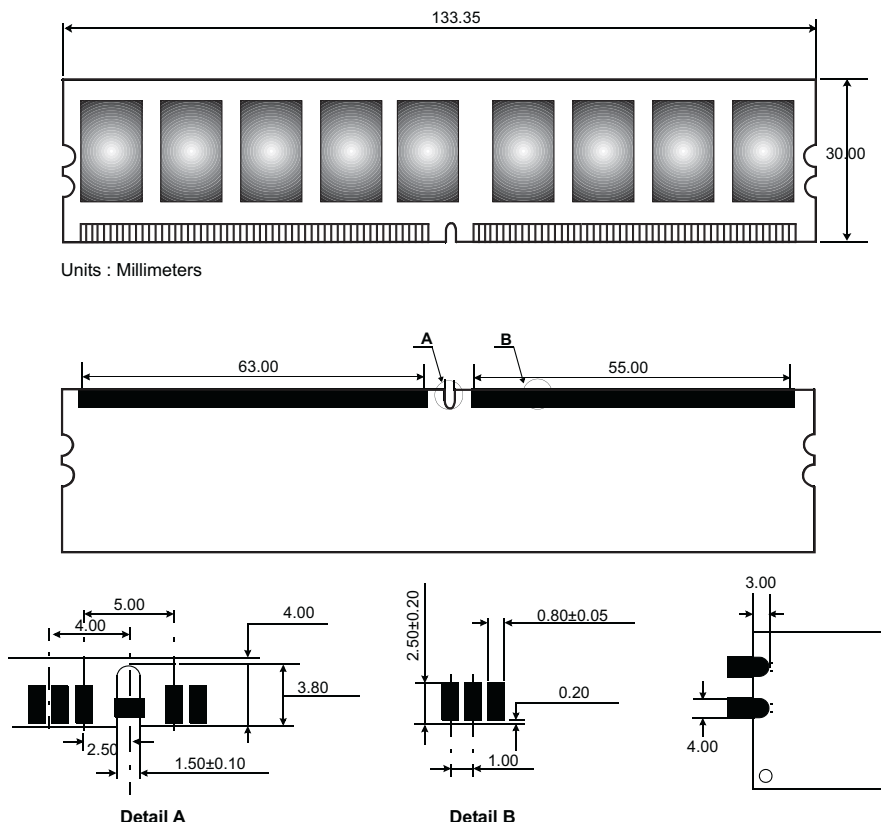
Figure 1: KVR667D2E5K2/512 240-Pin DIMM Kit
