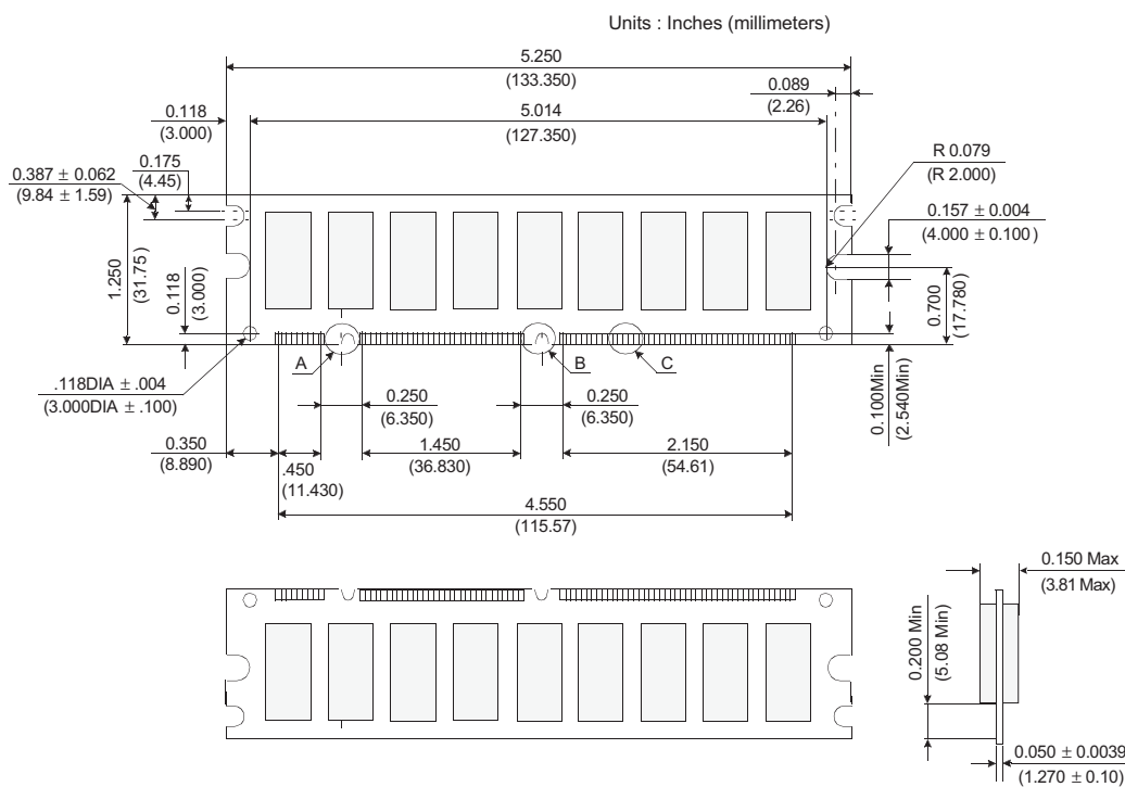
Figure 1: KVR100X72C3/512 168-Pin SDRAM Module
