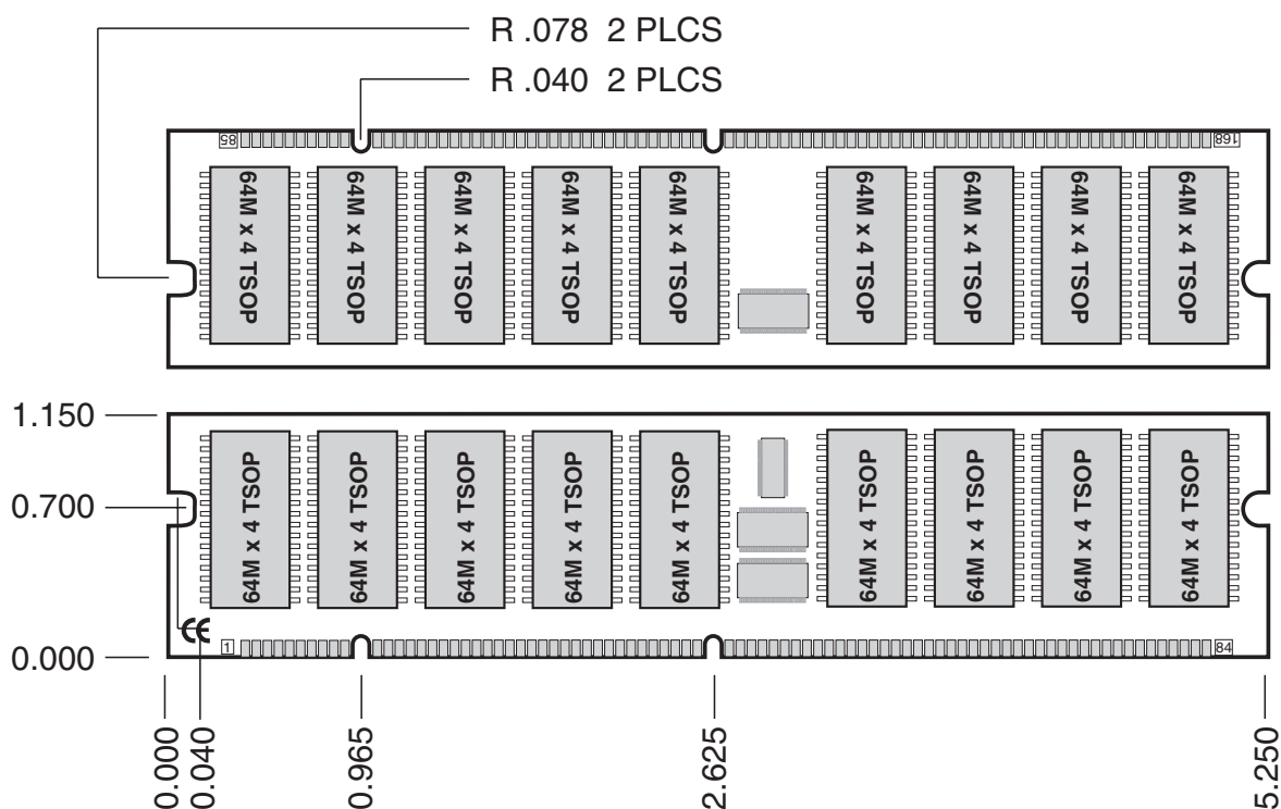
Figure 1: KVR133X72RC3L/512 168-Pin SDRAM Module
