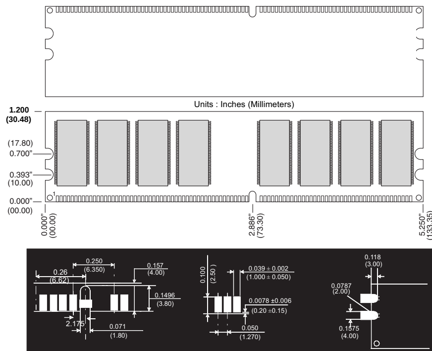
Figure 1: KVR333X64C25K2/512 184-Pin DIMM
