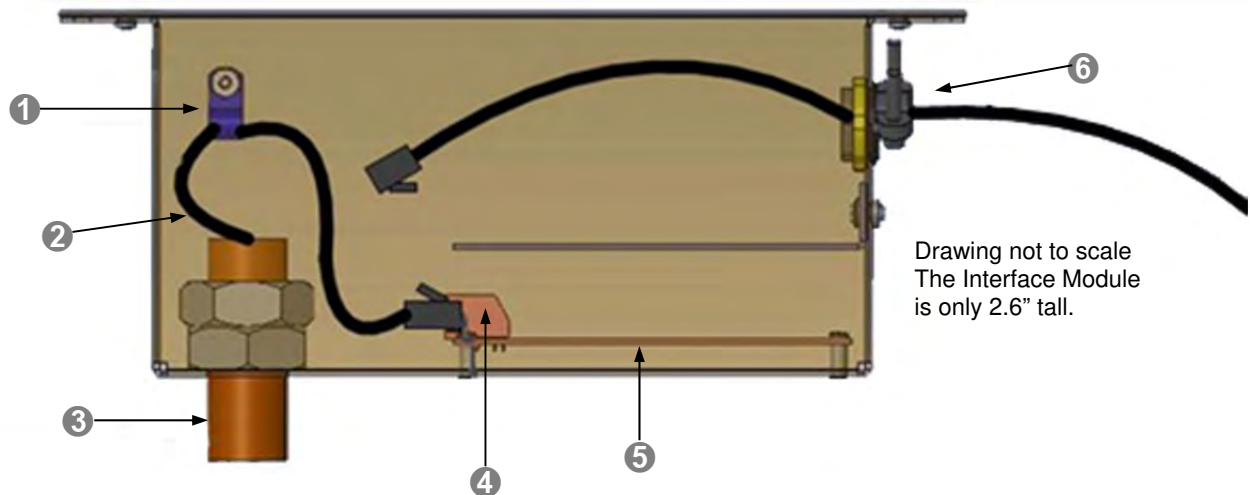
Diagram: TRIO Ceiling Mic Interface Module
