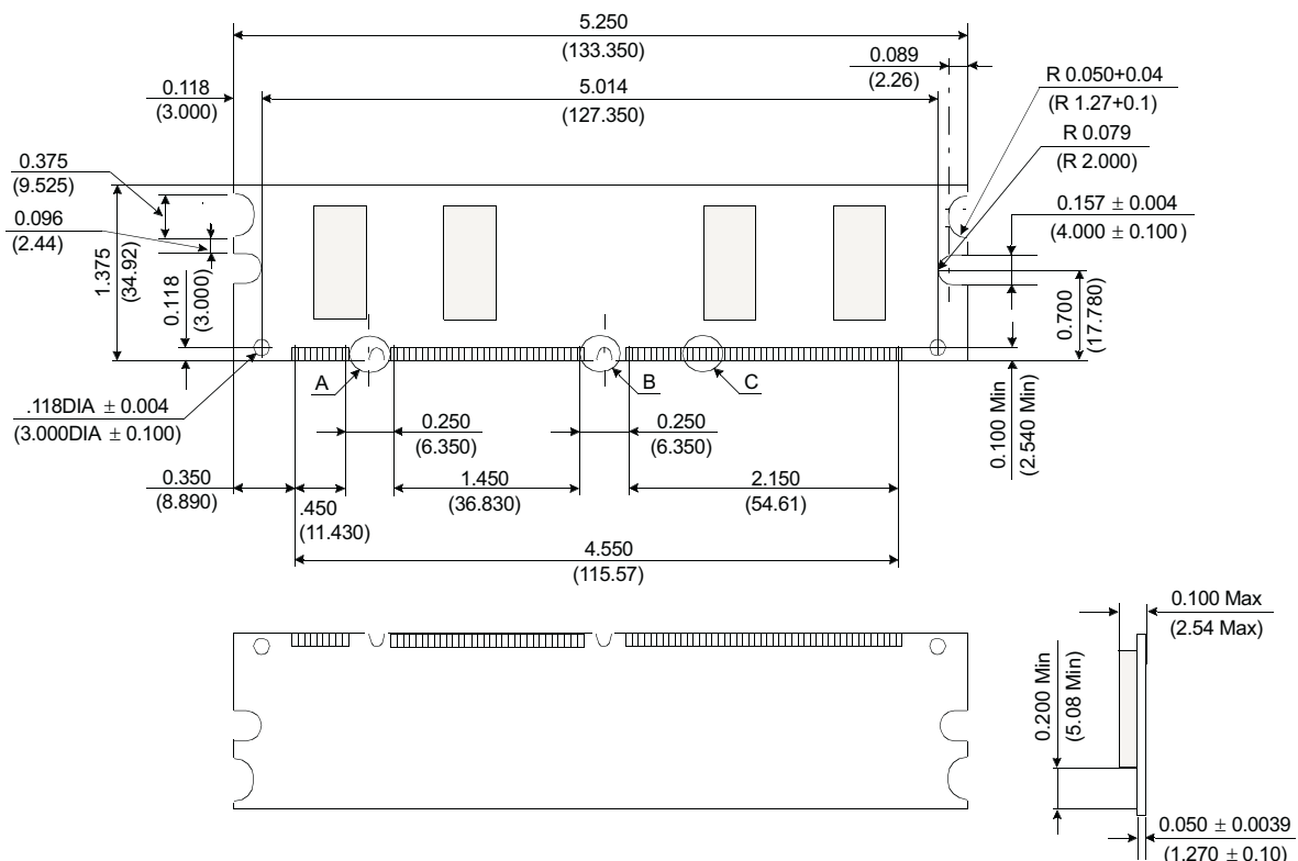
Figure 1: KVR133X64C3/128 168-Pin SDRAM Module
