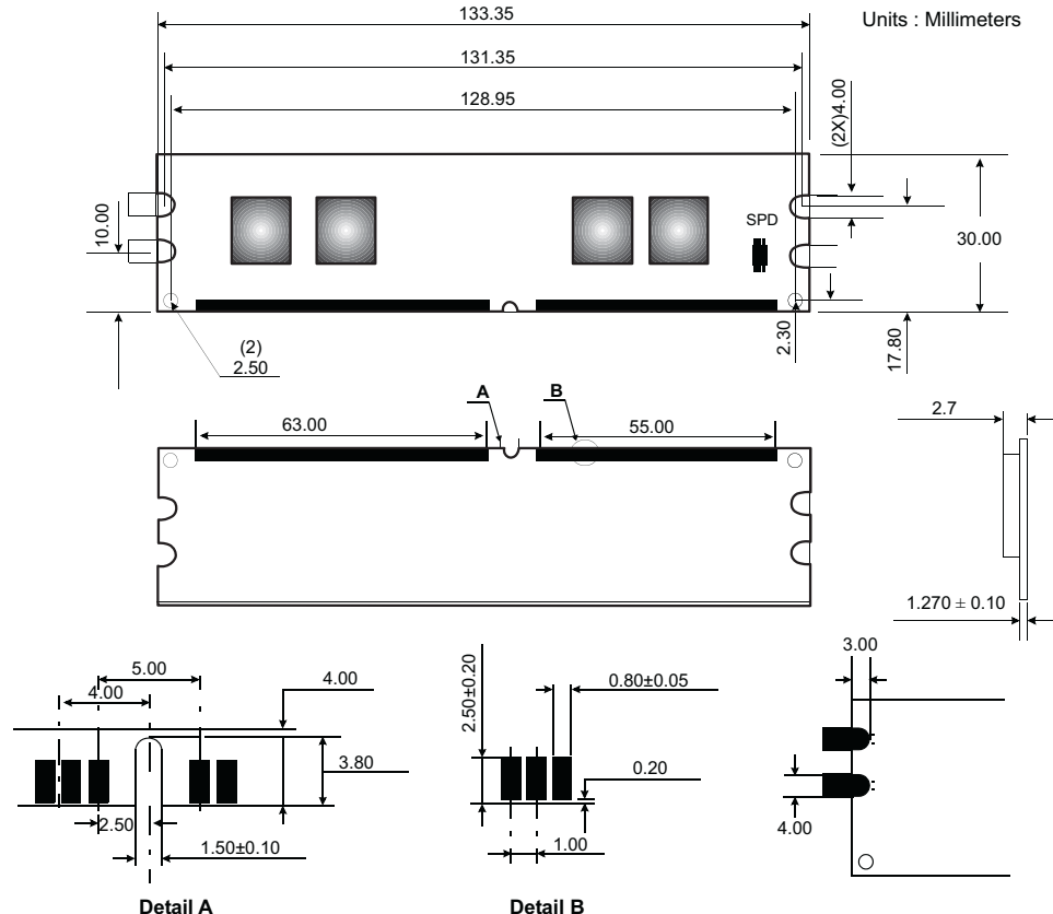
Figure 1: KVR400D2N3/256 240-Pin DIMM
