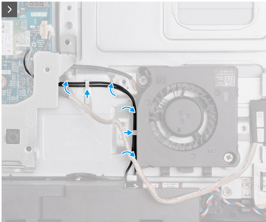
Figure 55. Installing the power-supply fan
