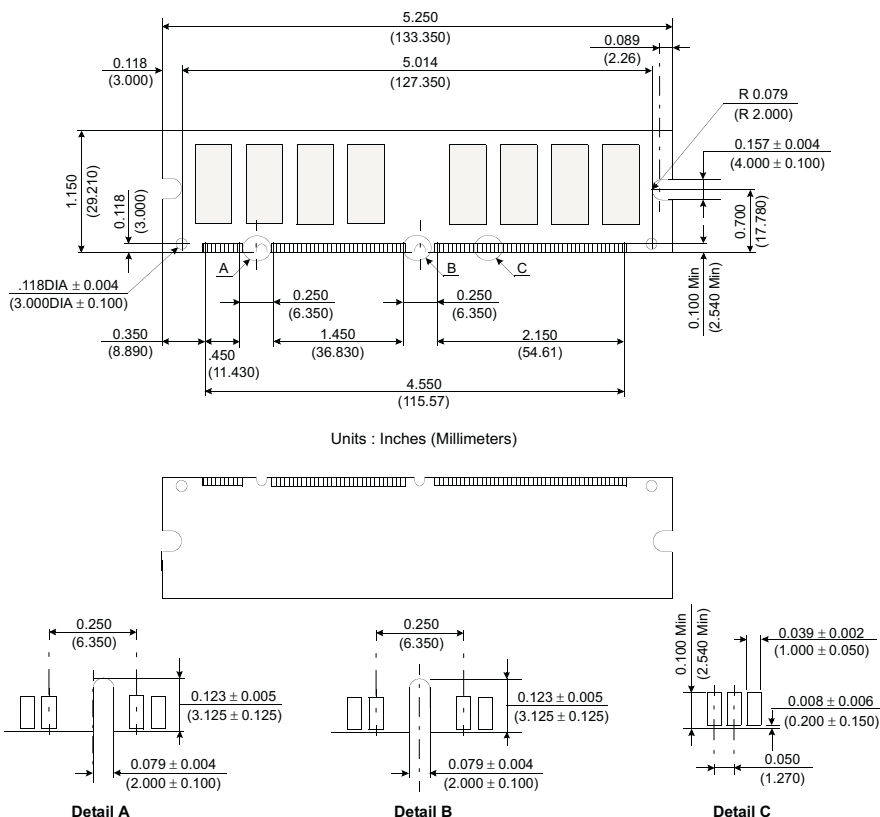
Figure 1: KVR133X64C2/256 168-Pin SDRAM Module
