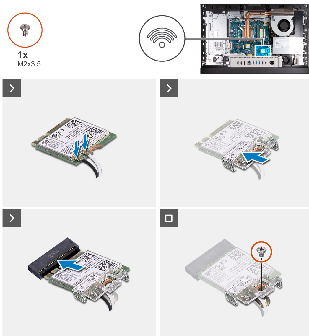
Figure 29. Installing the wireless card
