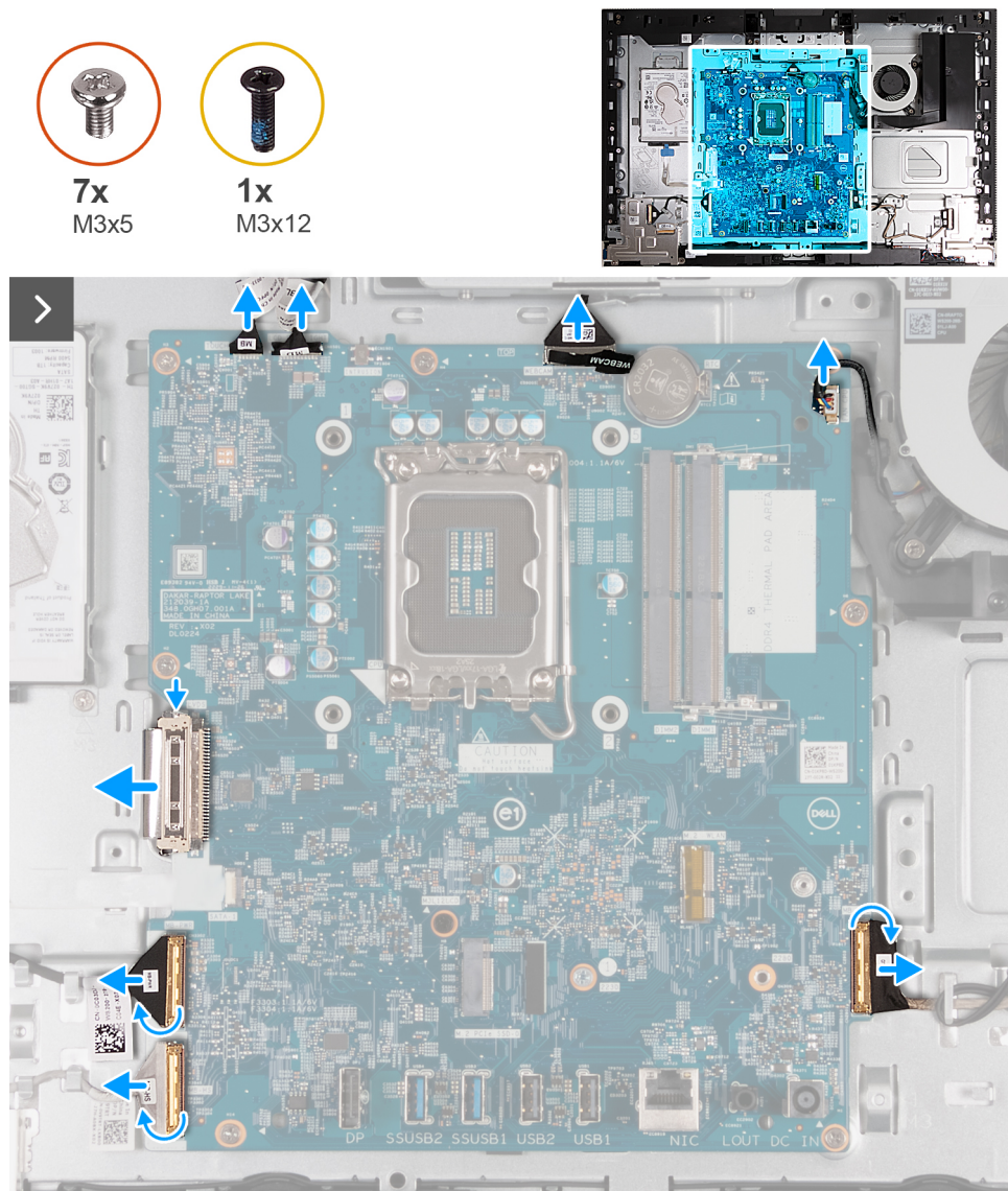
Figure 114. Removing the system board
