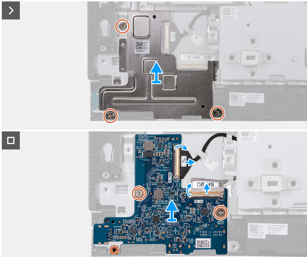
Figure 72. Removing the power-button and I/O board
