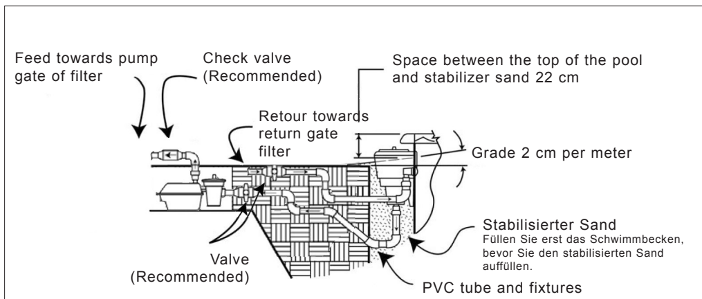
FIG. 2 SPECIFIC INSTALLATION
